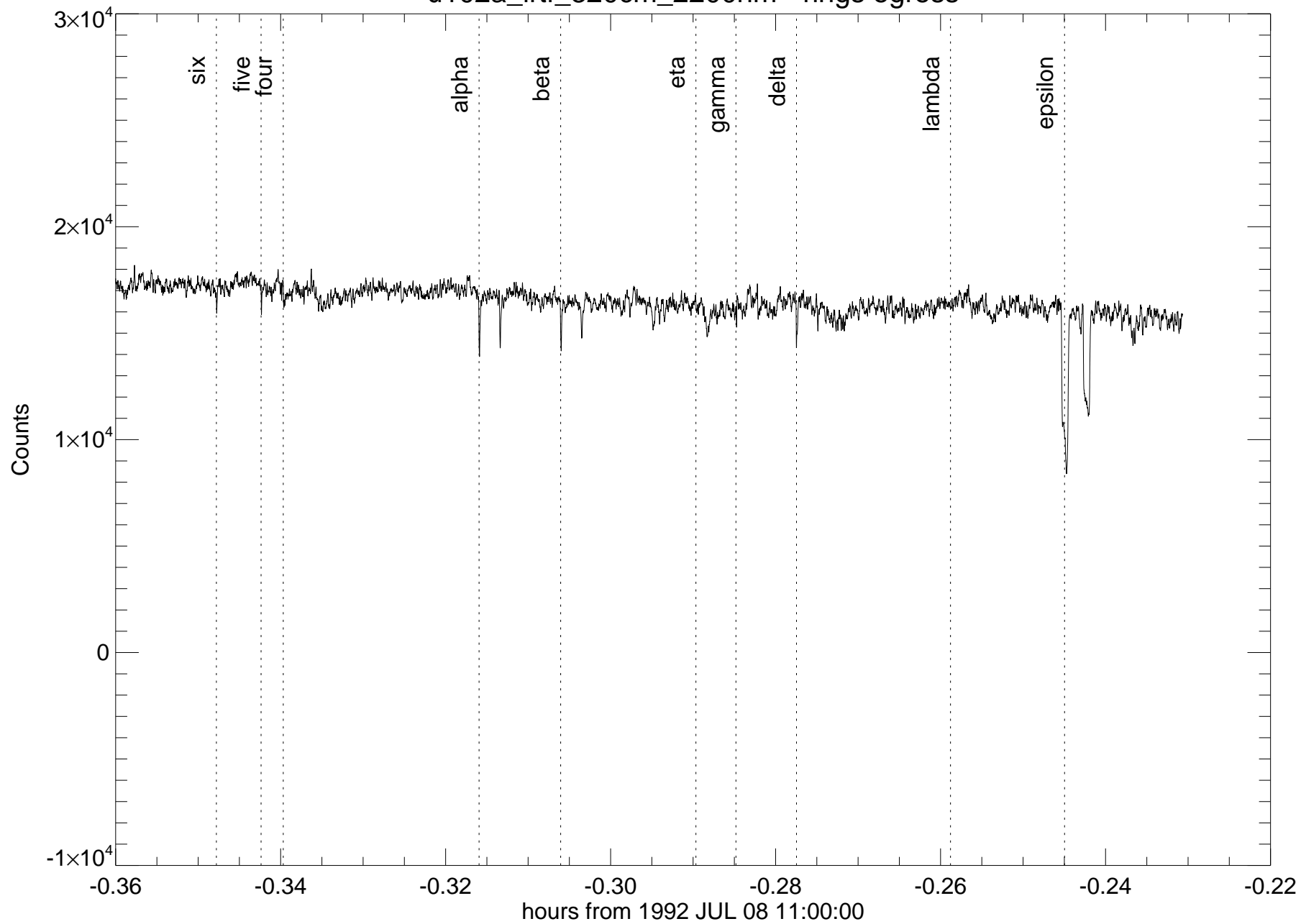
u102a_irtf_320cm_2200nm - rings egress
