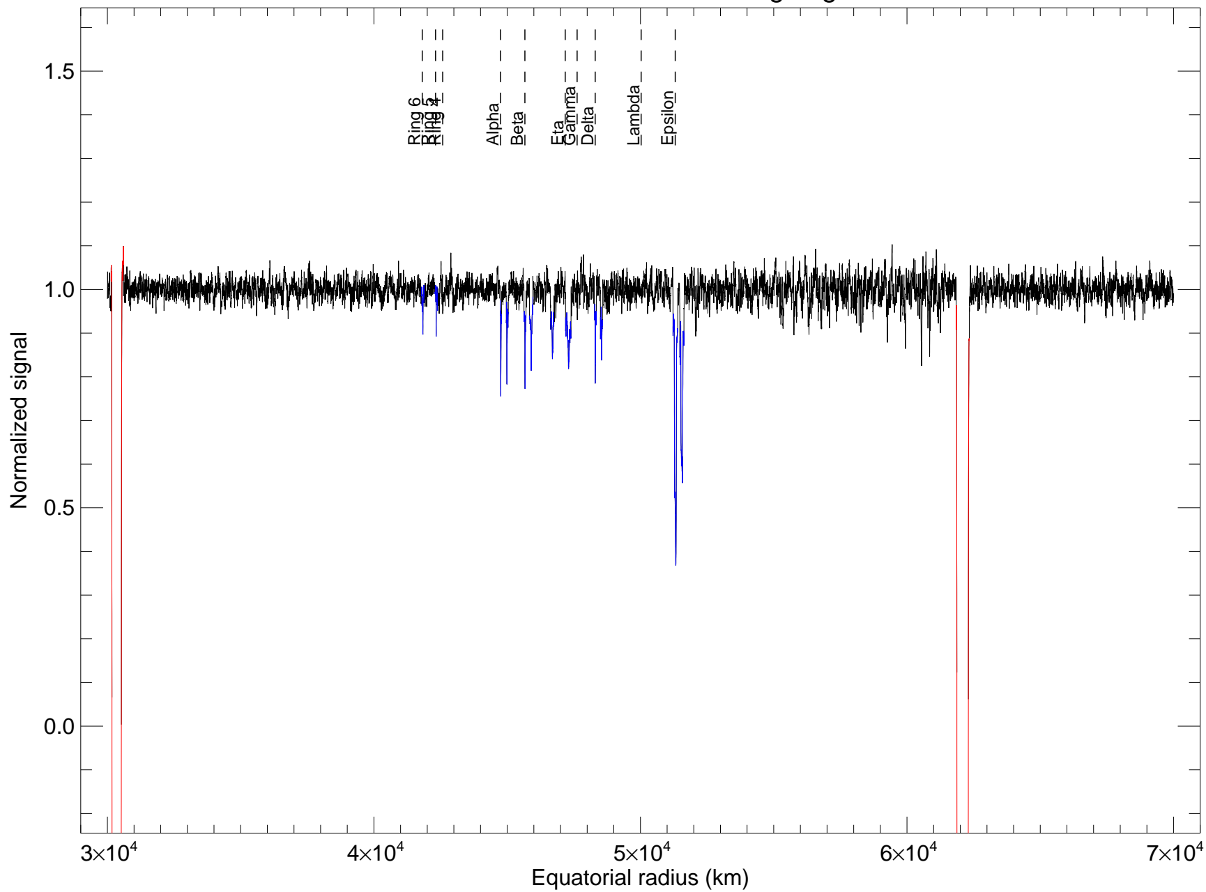
u102a_irtf_320cm_2200nm rings egress
