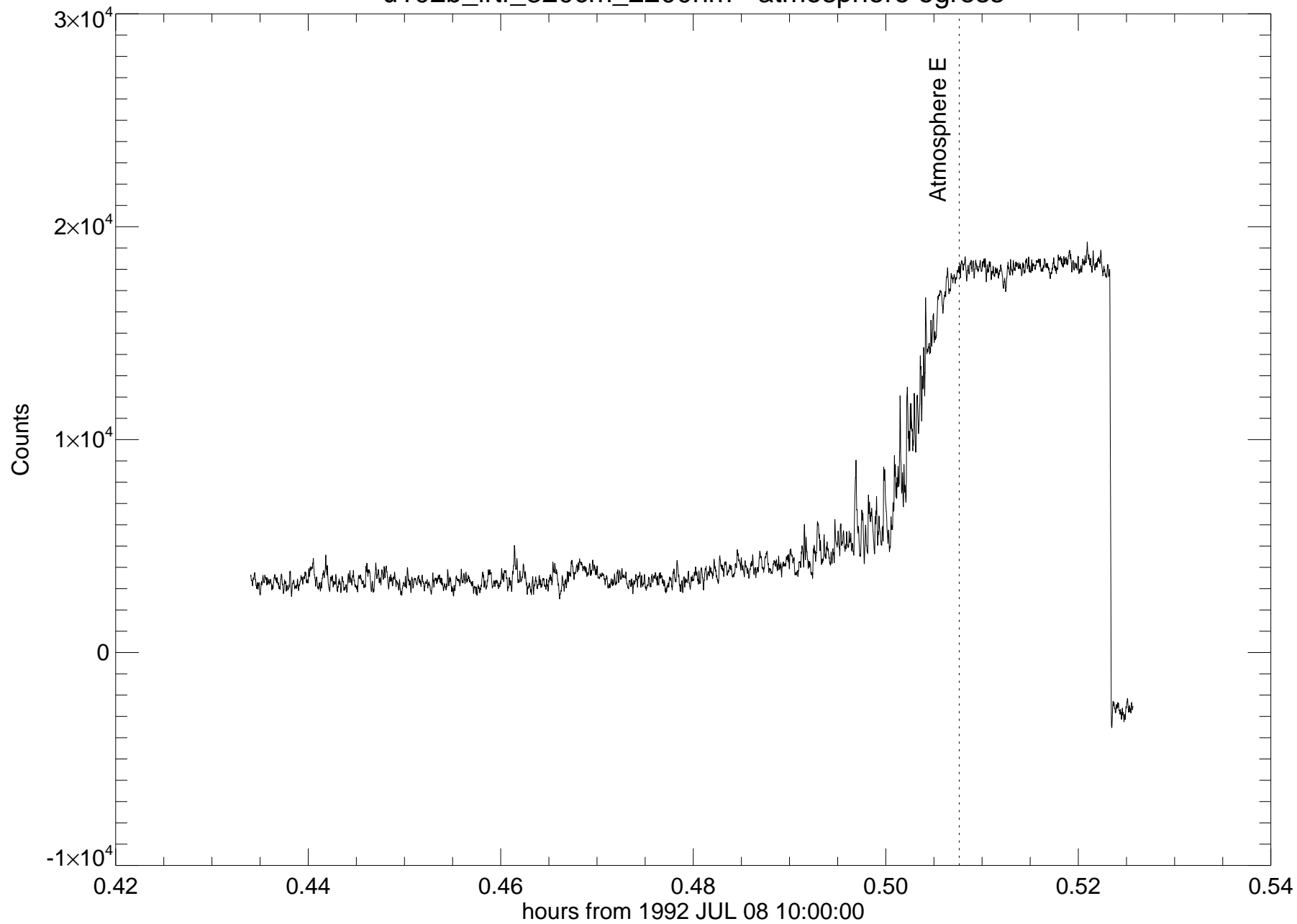
u102b_irtf_320cm_2200nm - atmosphere egress
