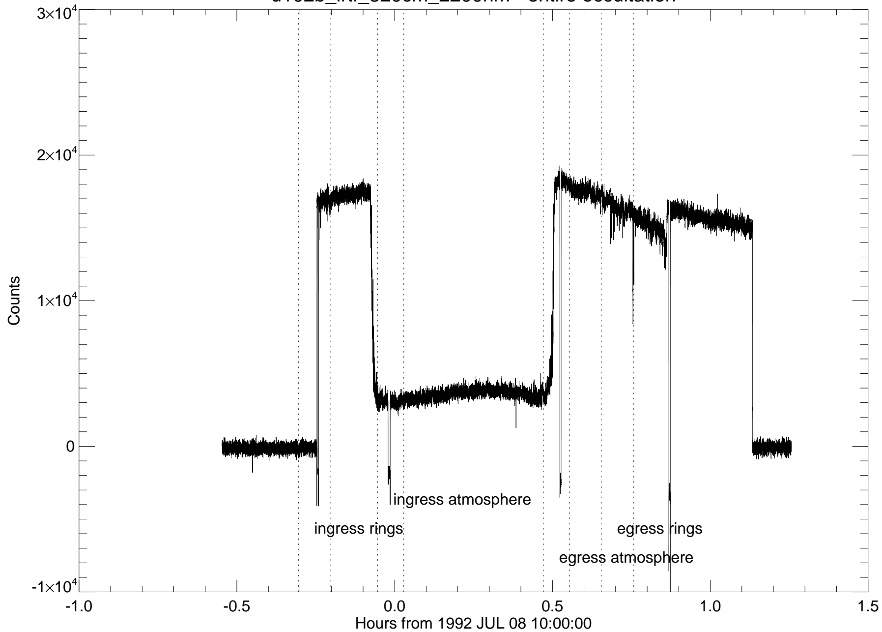
u102b_irtf_320cm_2200nm - entire occultation
