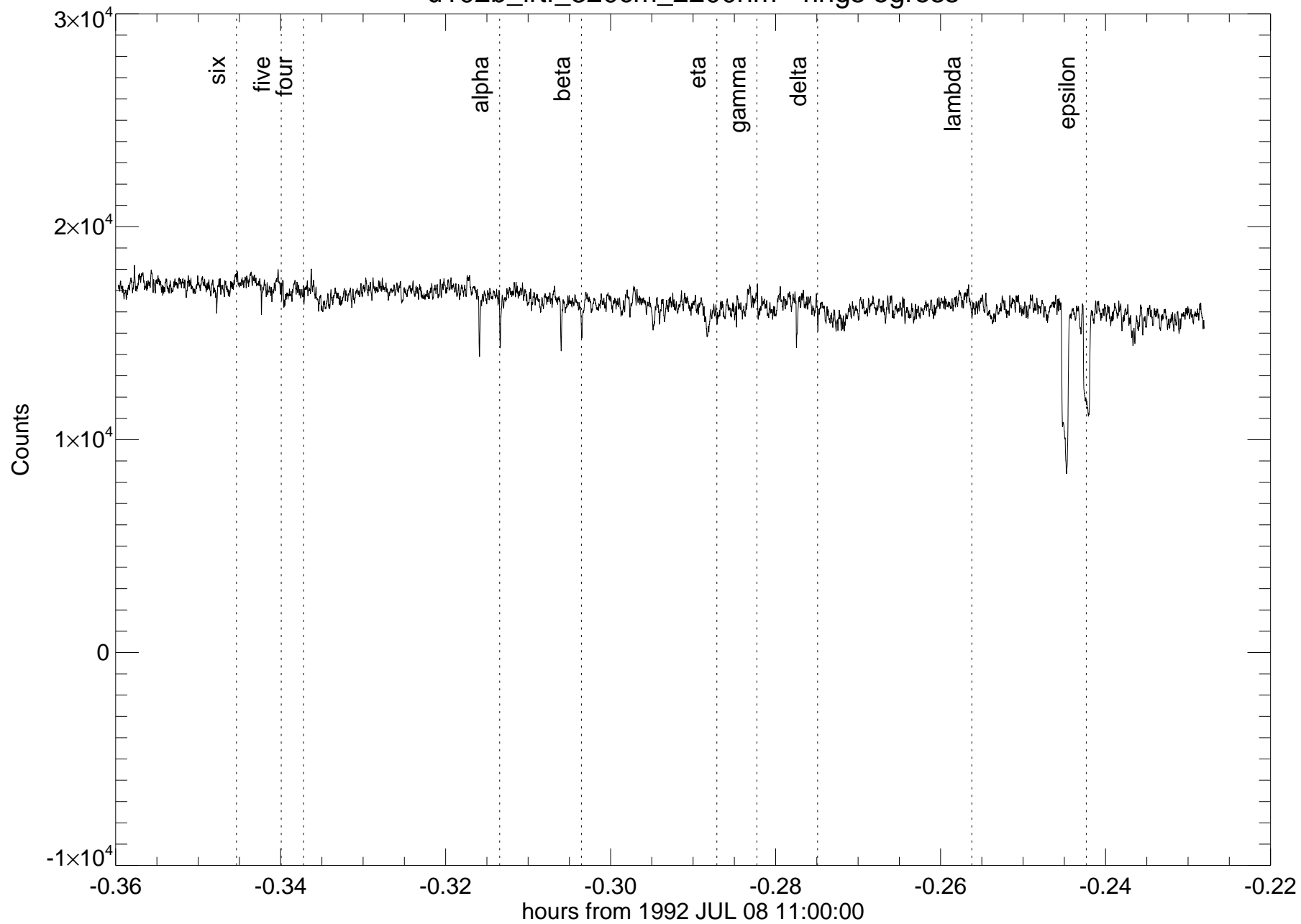
u102b_irtf_320cm_2200nm - rings egress
