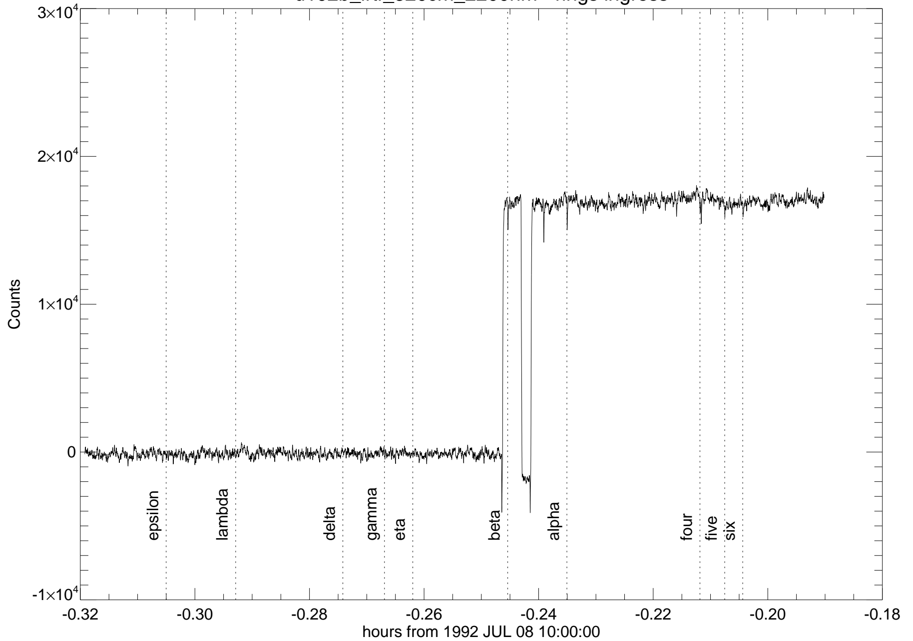
u102b_irtf_320cm_2200nm - rings ingress
