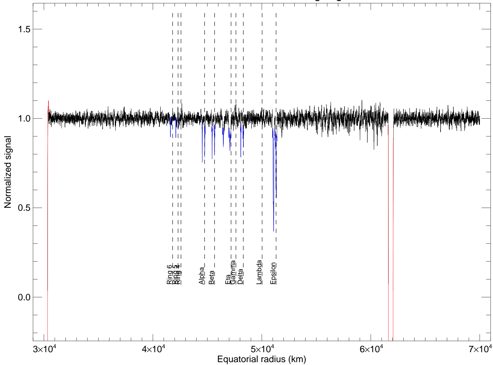
u102b_irtf_320cm_2200nm rings egress
