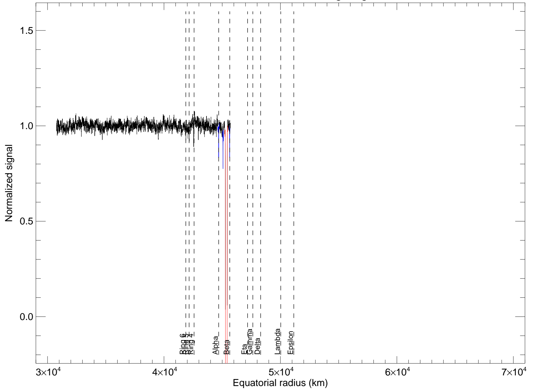
u102b_irtf_320cm_2200nm rings ingress
