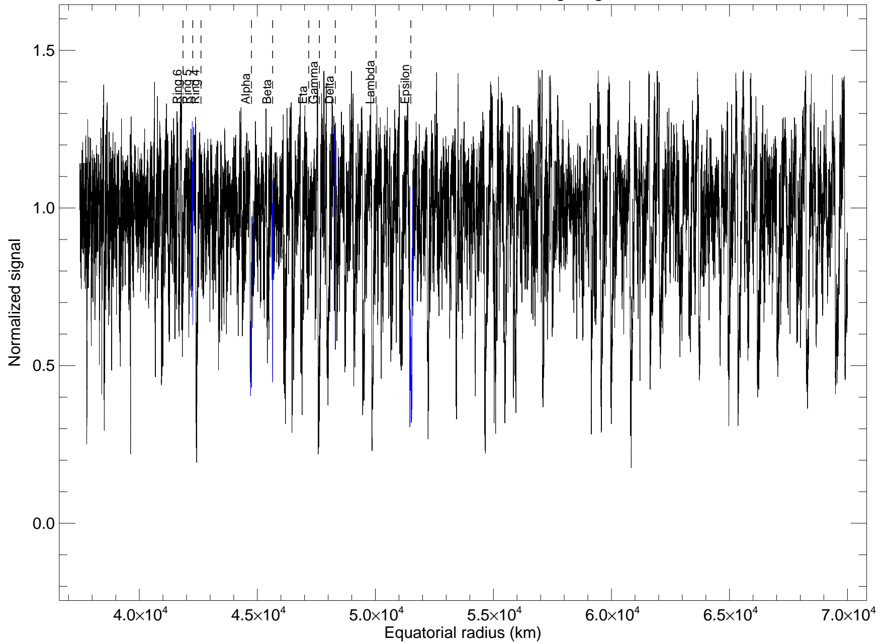
u103_eso_220cm_2200nm rings egress
