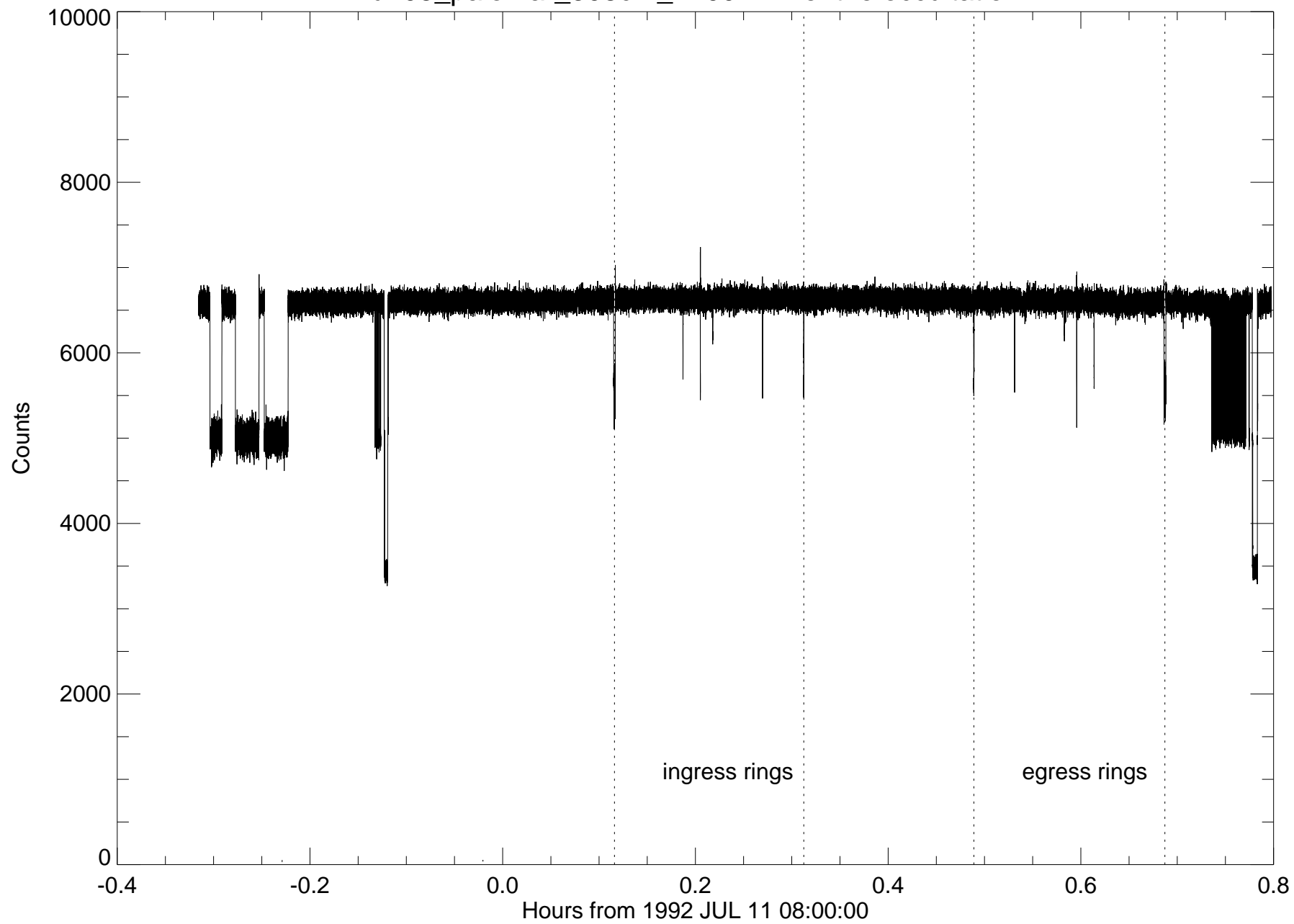
u103_palomar_508cm_2200nm - entire occultation
