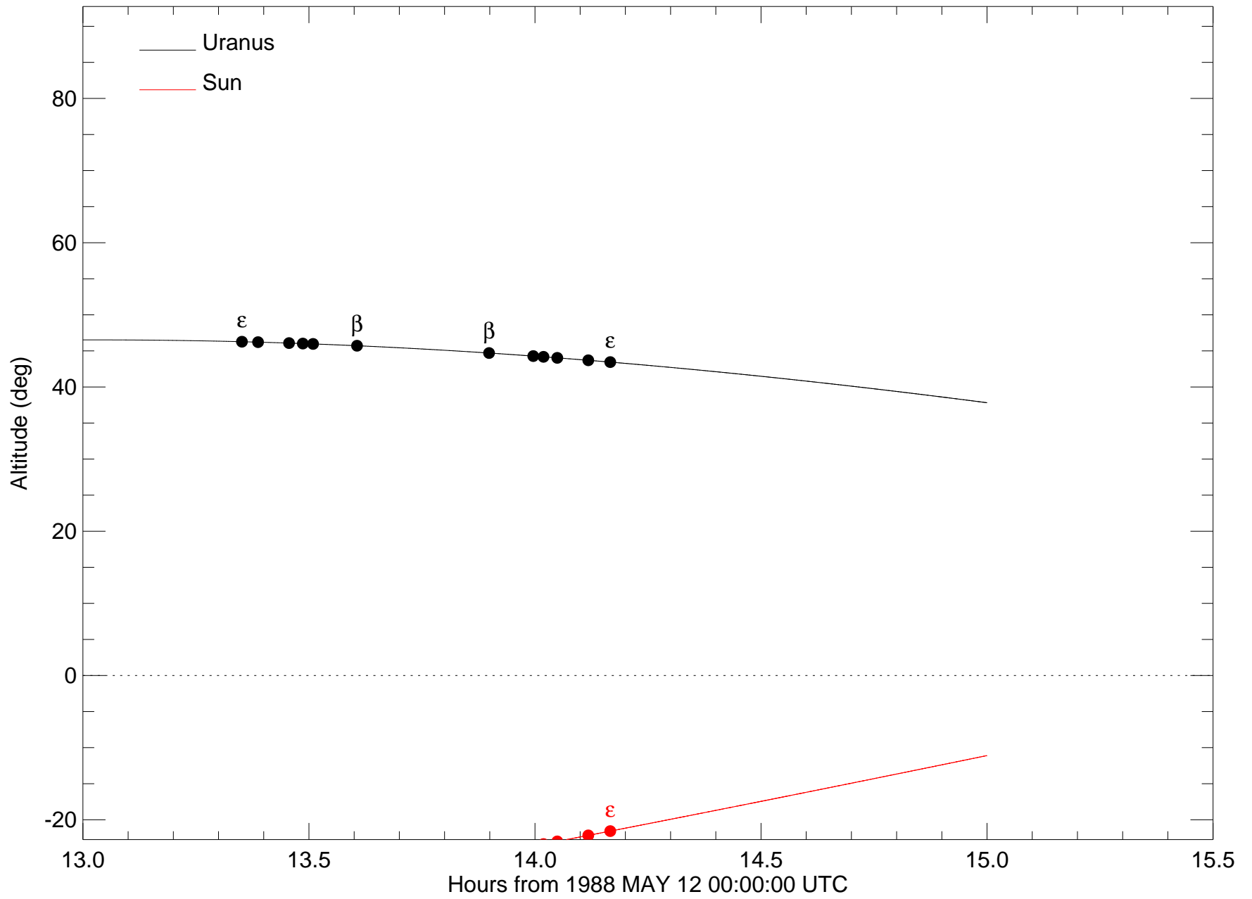
u1052 observed from IRTF 320cm
