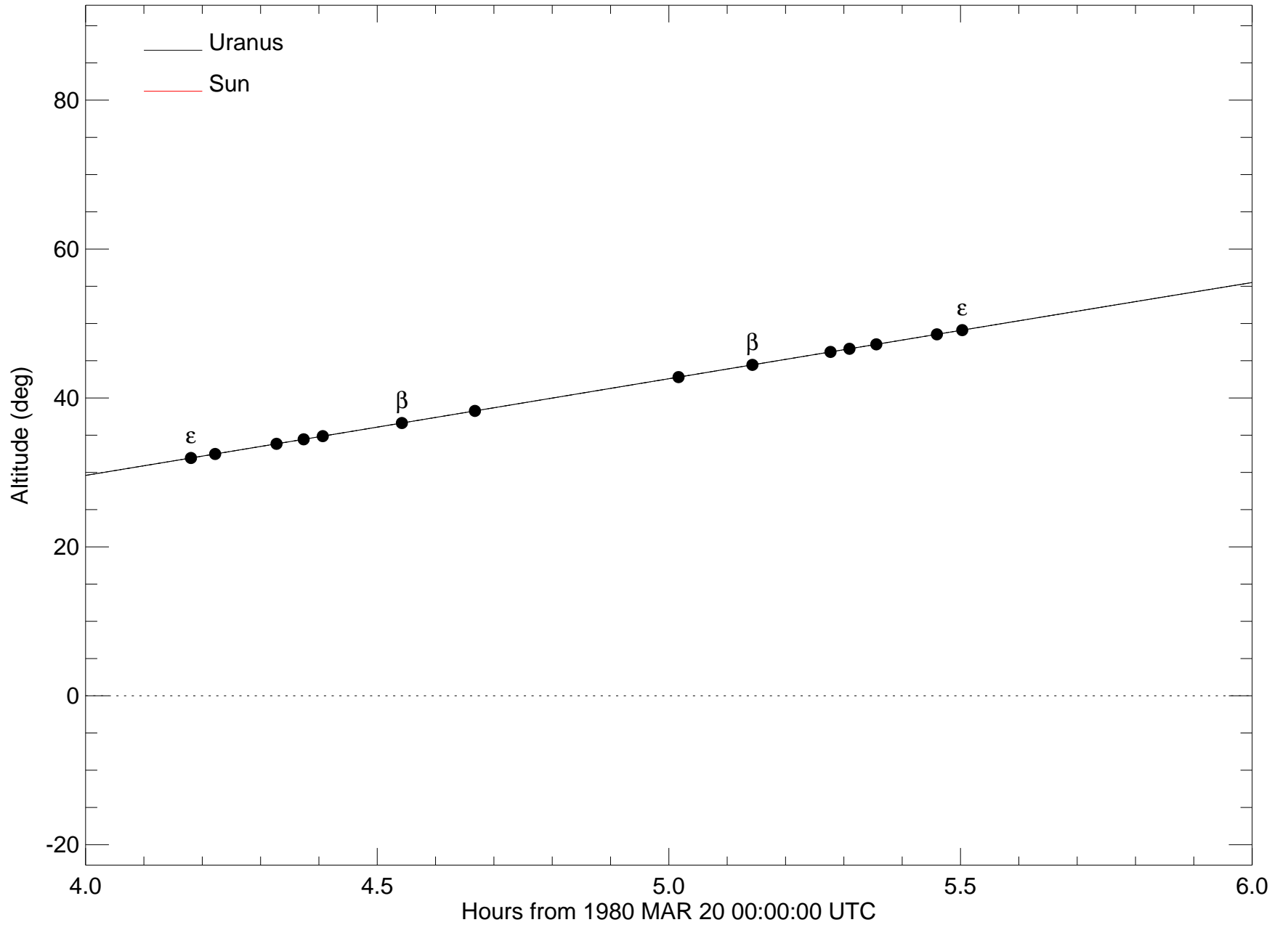
u11 observed from Cerro Tololo Inter-American Observatory 400cm
