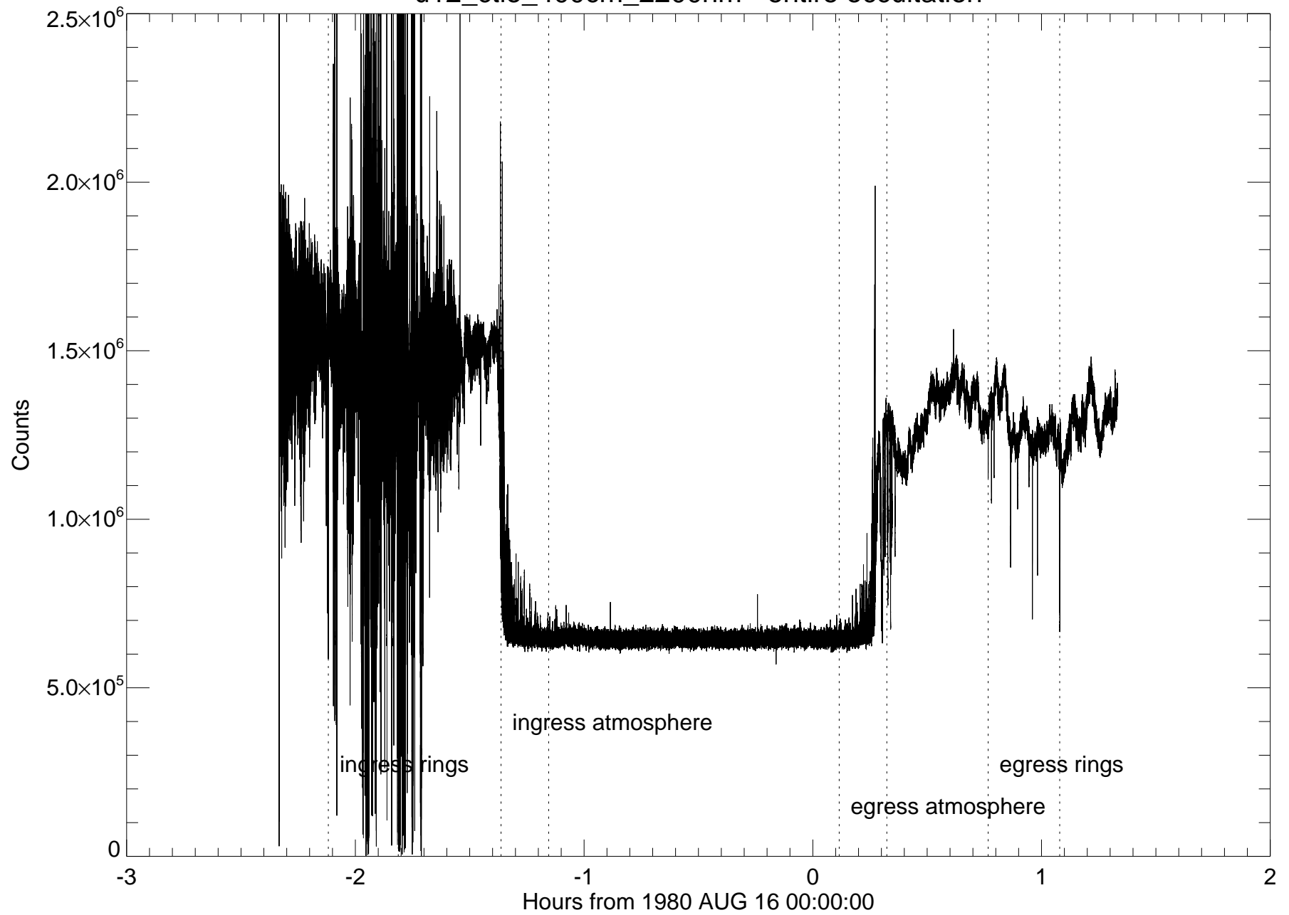
u12_ctio_400cm_2200nm - entire occultation
