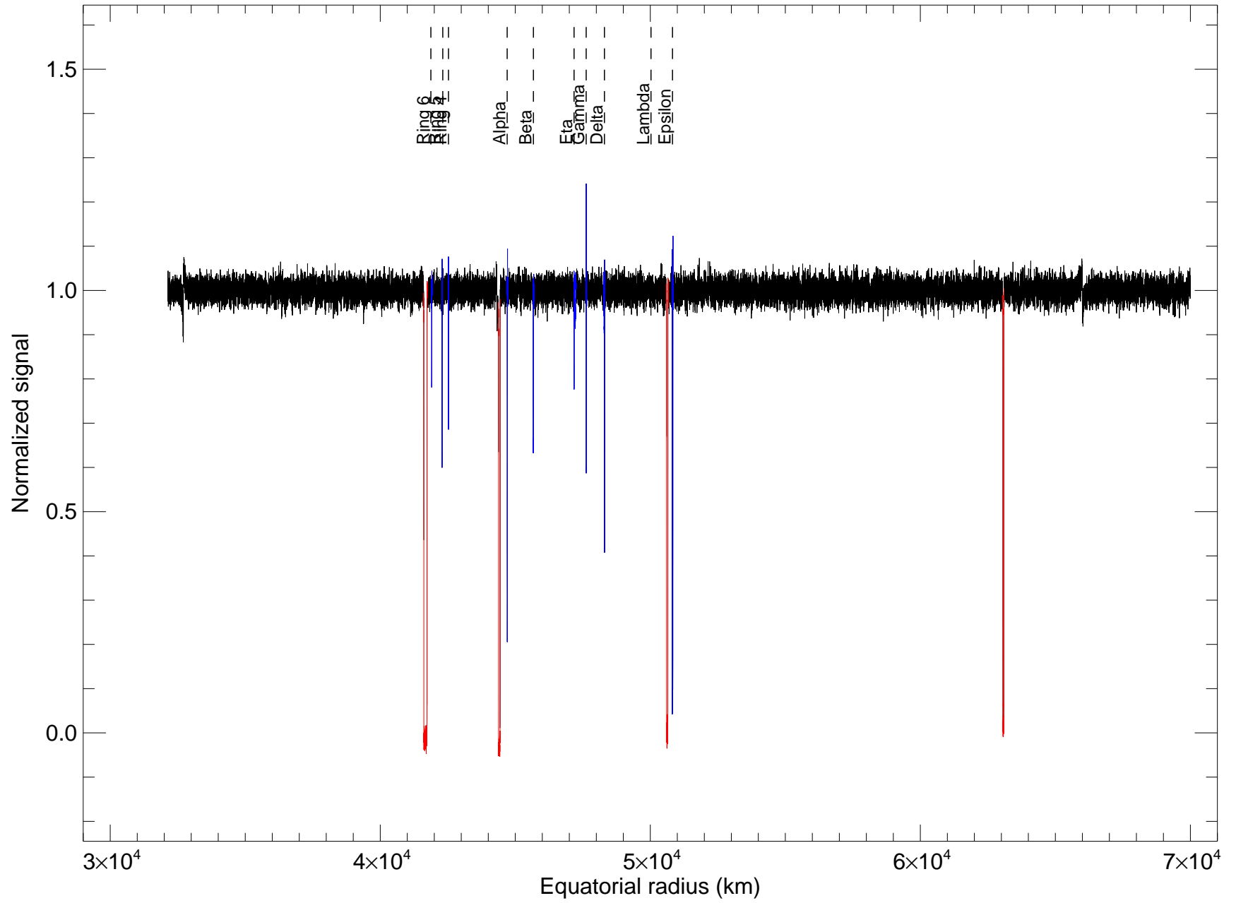
u134_saao_188cm_2220nm rings ingress
