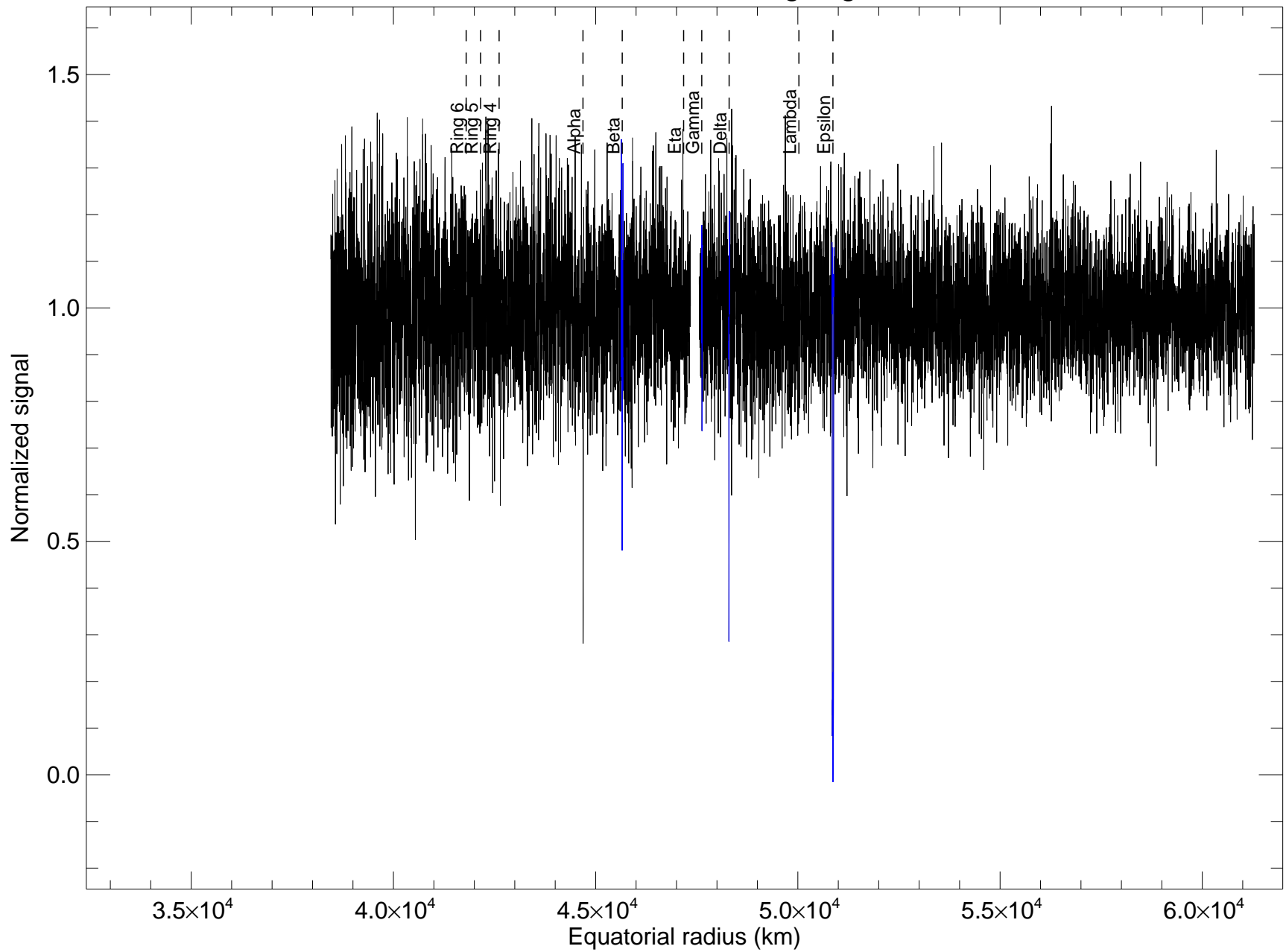
u137_hst_fos_540nm rings egress
