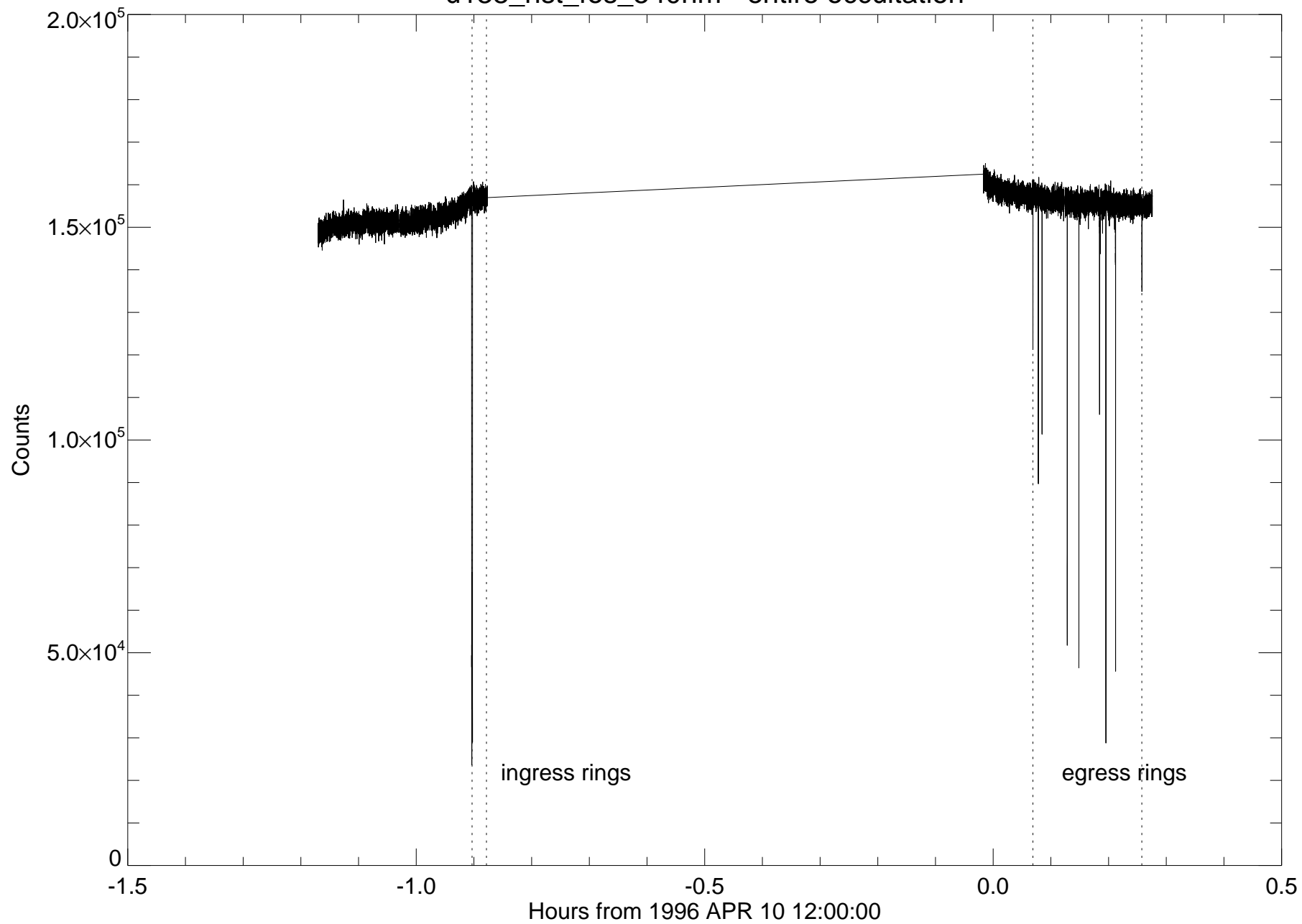
u138_hst_fos_540nm - entire occultation
