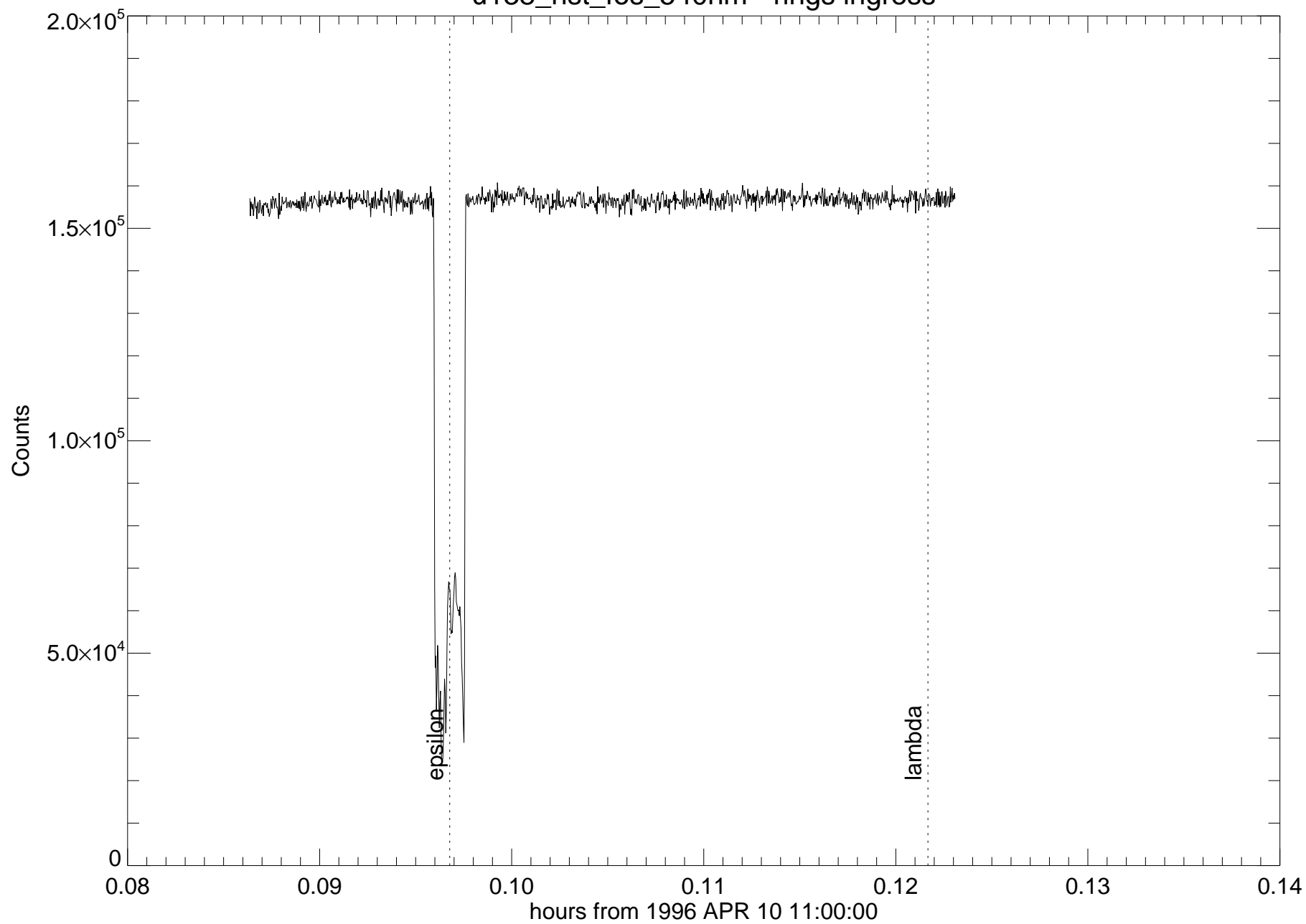
u138_hst_fos_540nm - rings ingress
