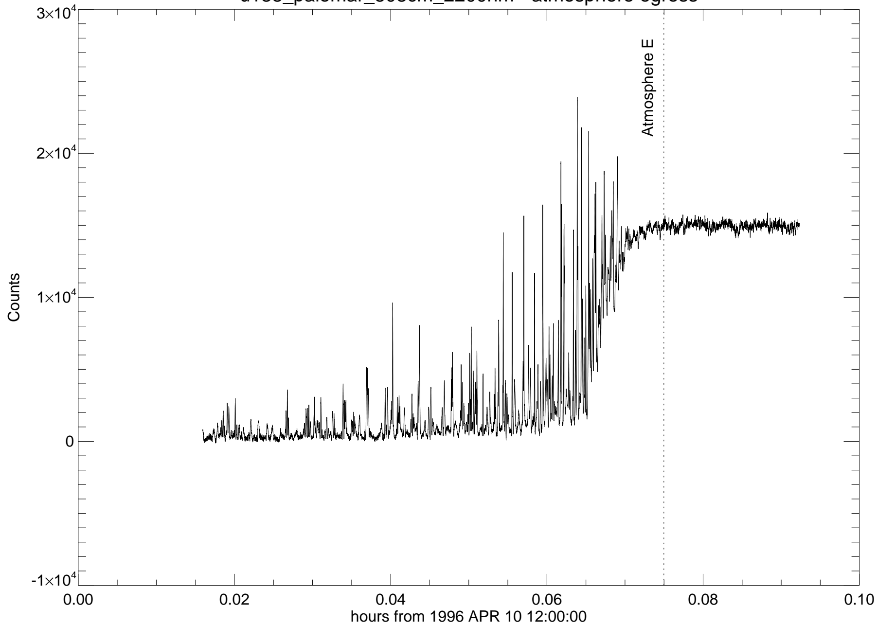
u138_palomar_508cm_2200nm - atmosphere egress
