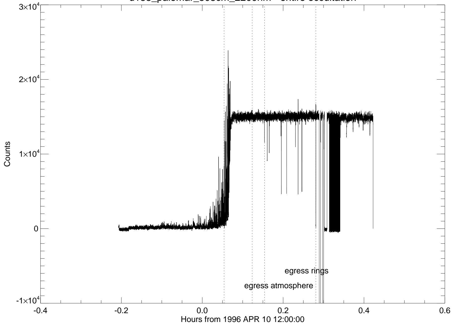
u138_palomar_508cm_2200nm - entire occultation
