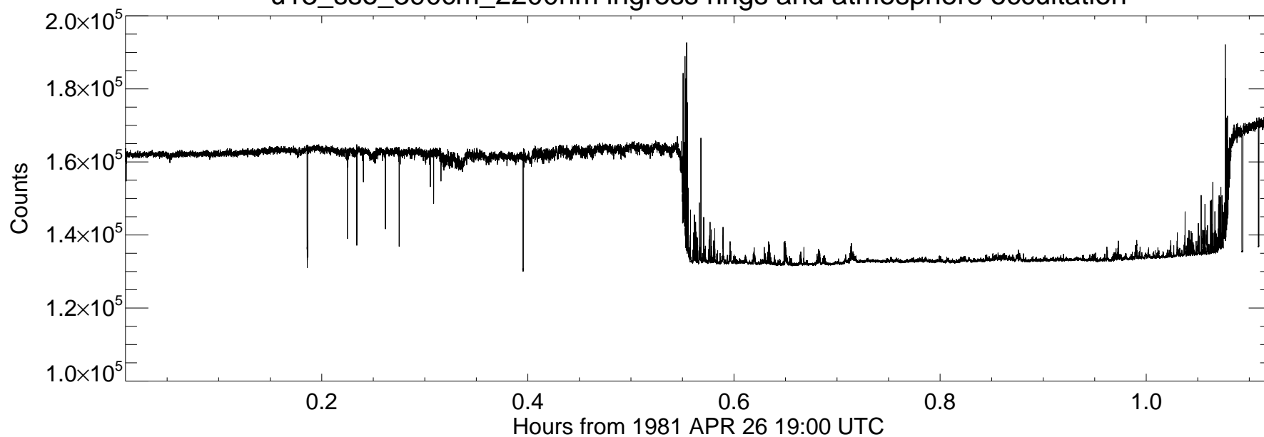
u13_sso_390cm_2200nm ingress rings and atmosphere occultation
