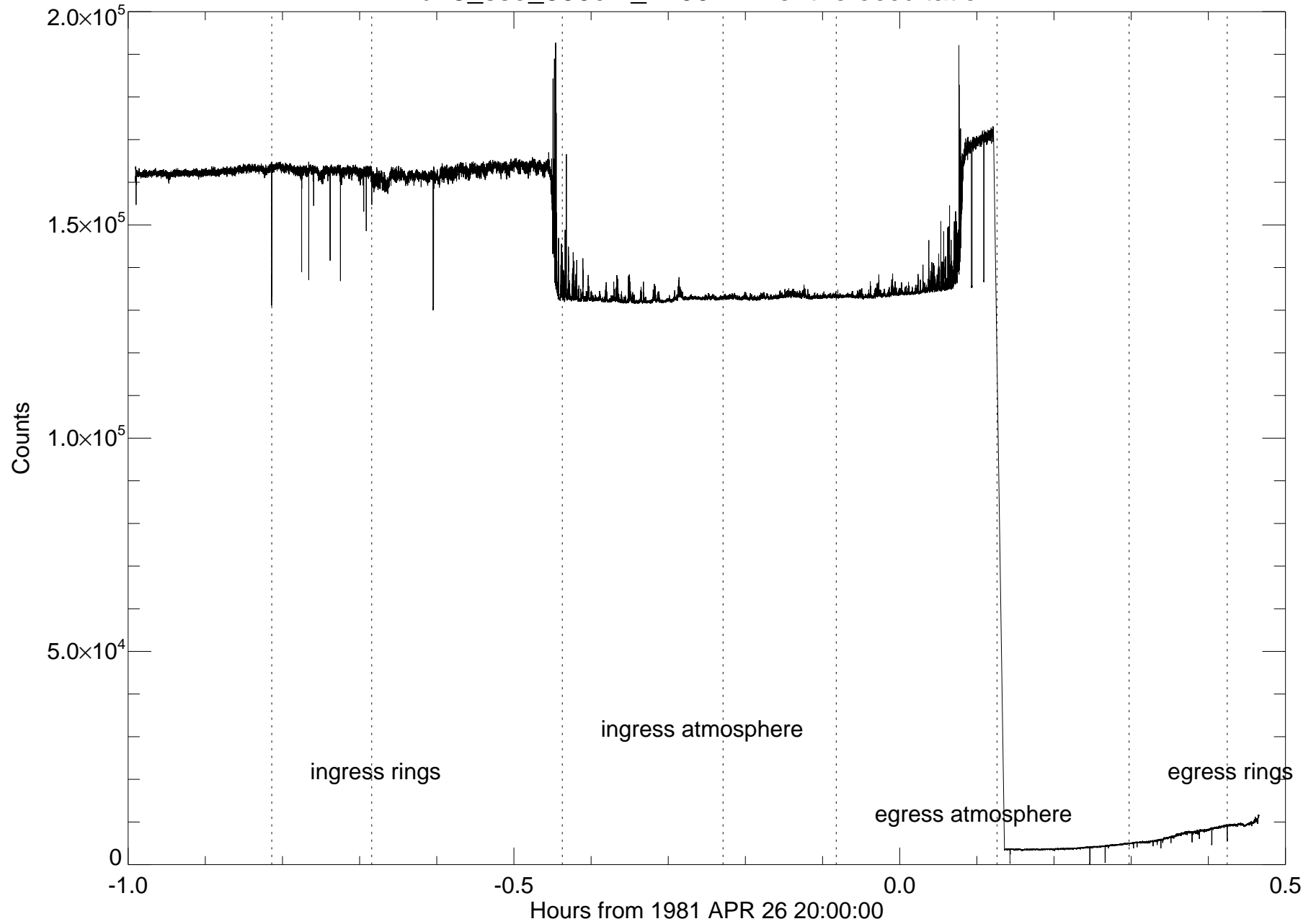
u13_sso_390cm_2200nm - entire occultation
