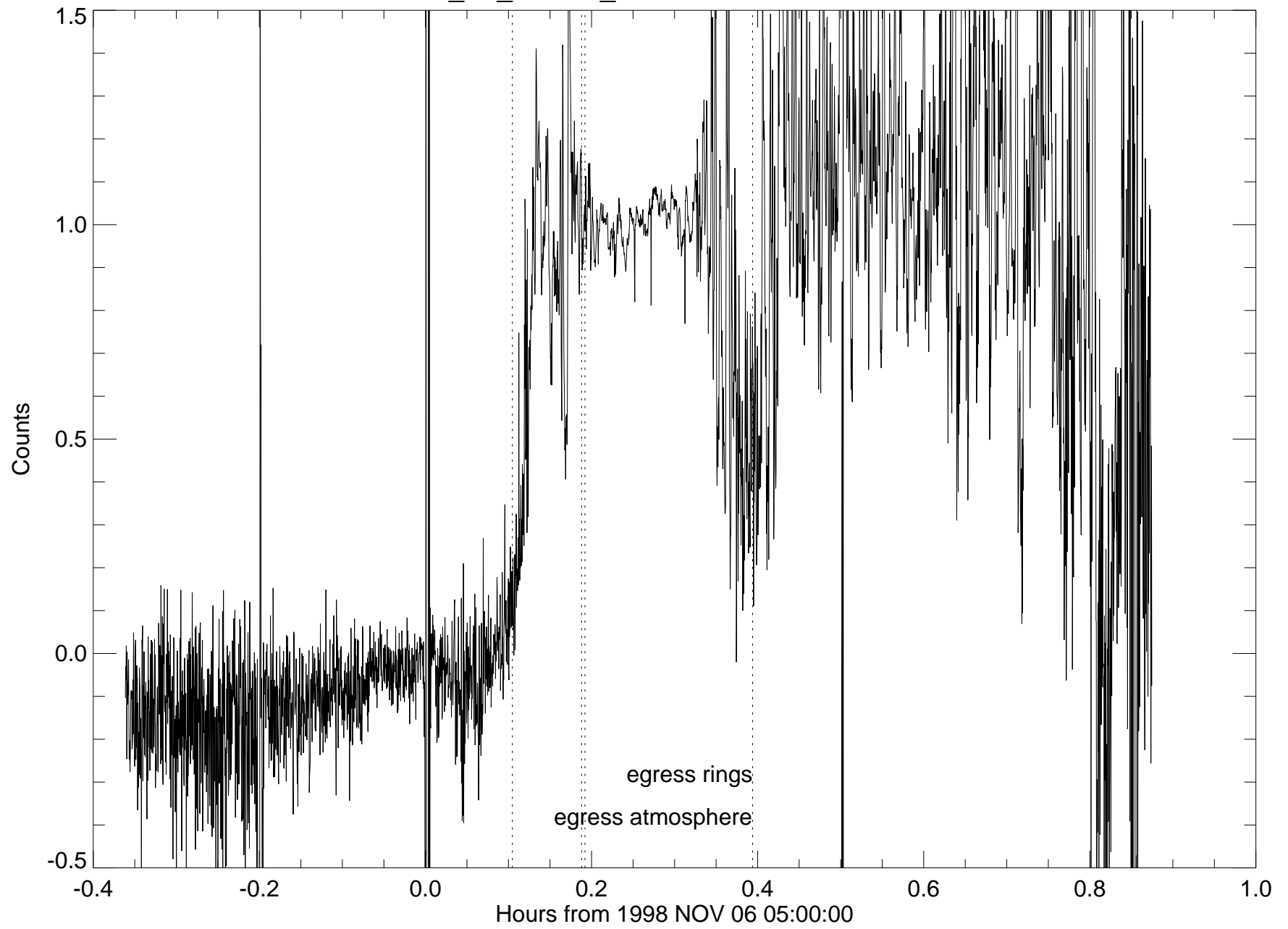
u149_irtf_320cm_2200nm - entire occultation
