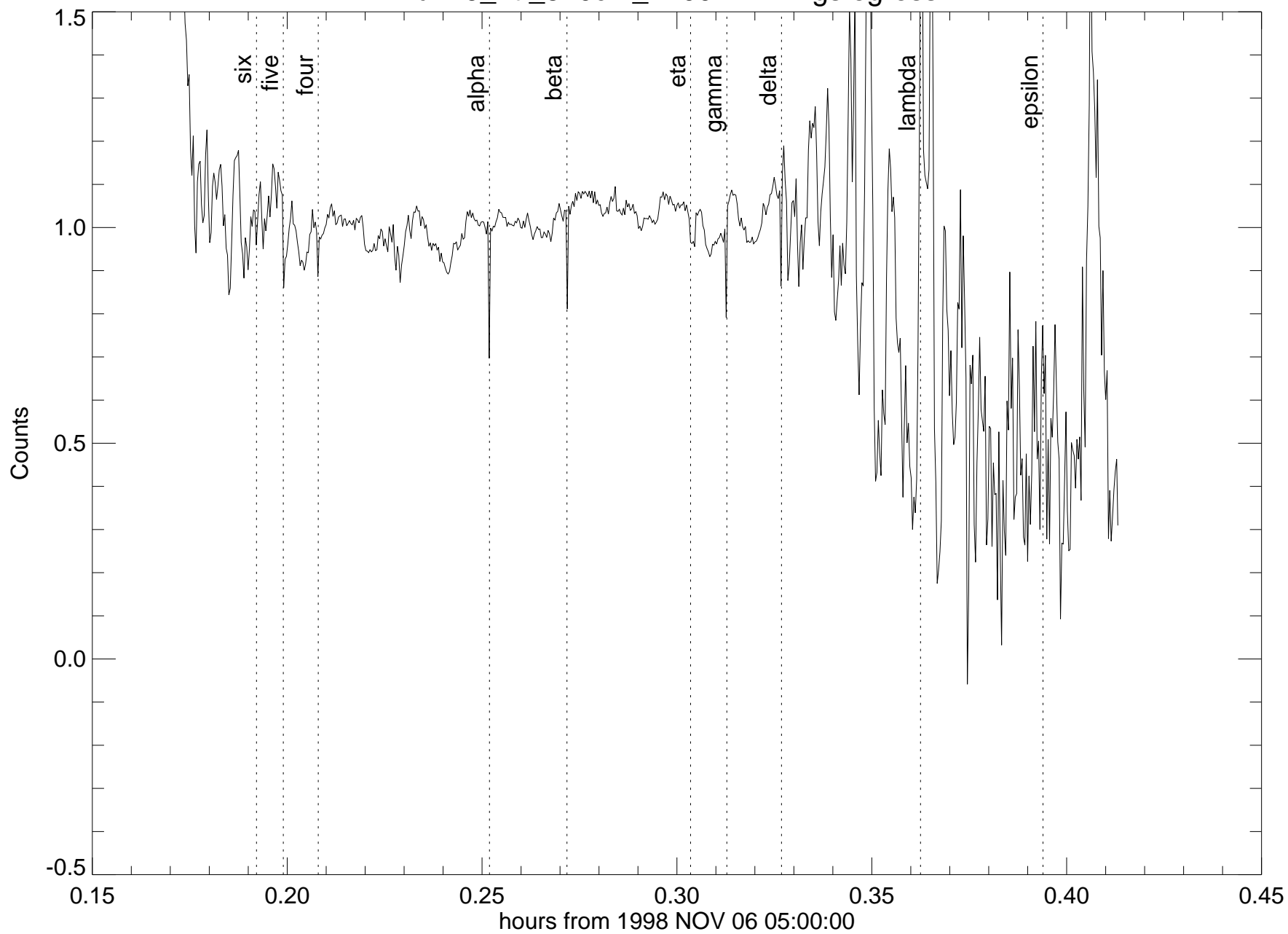
u149_irtf_320cm_2200nm - rings egress
