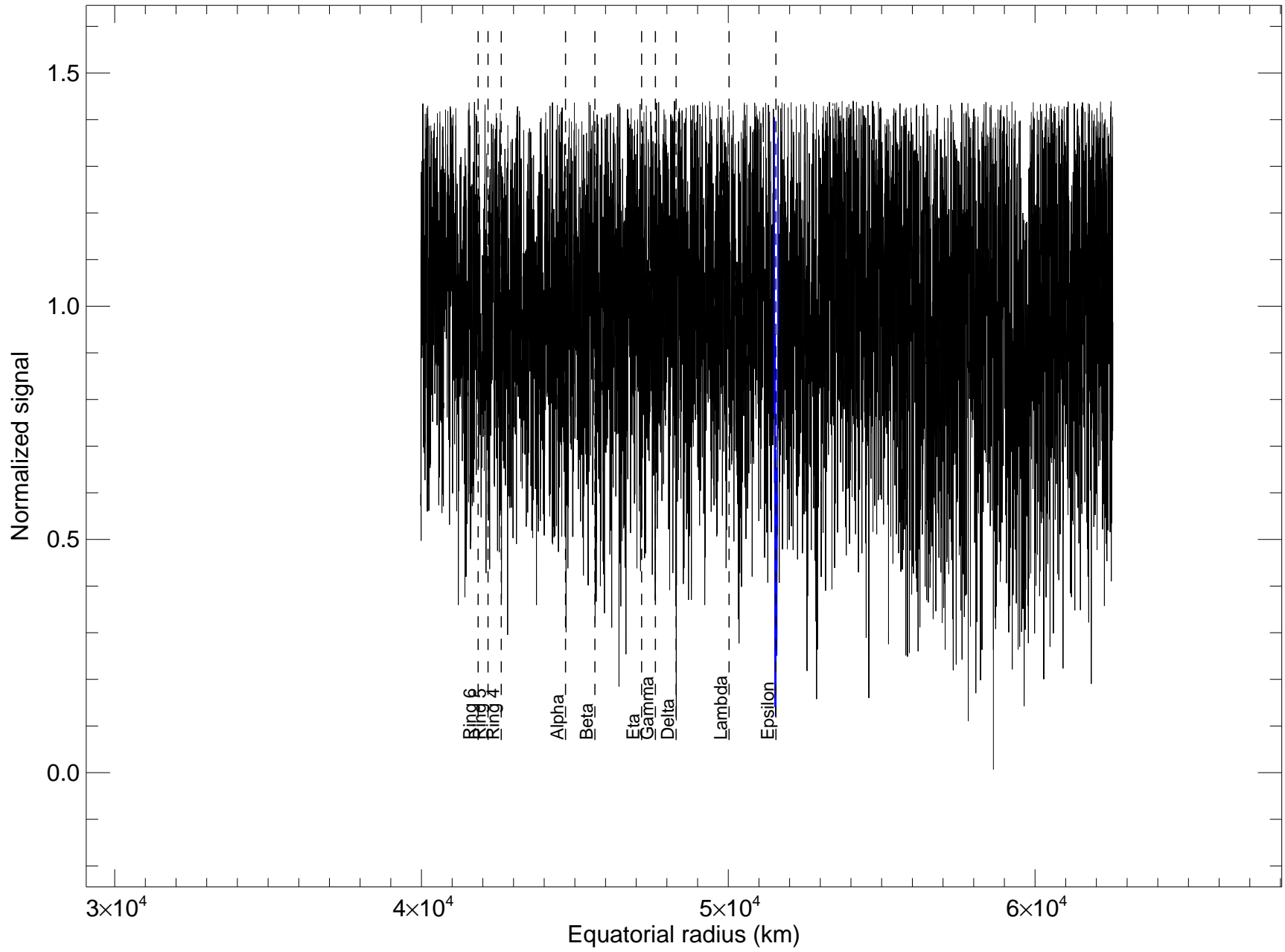
u149_lowell_180cm_890nm rings egress
