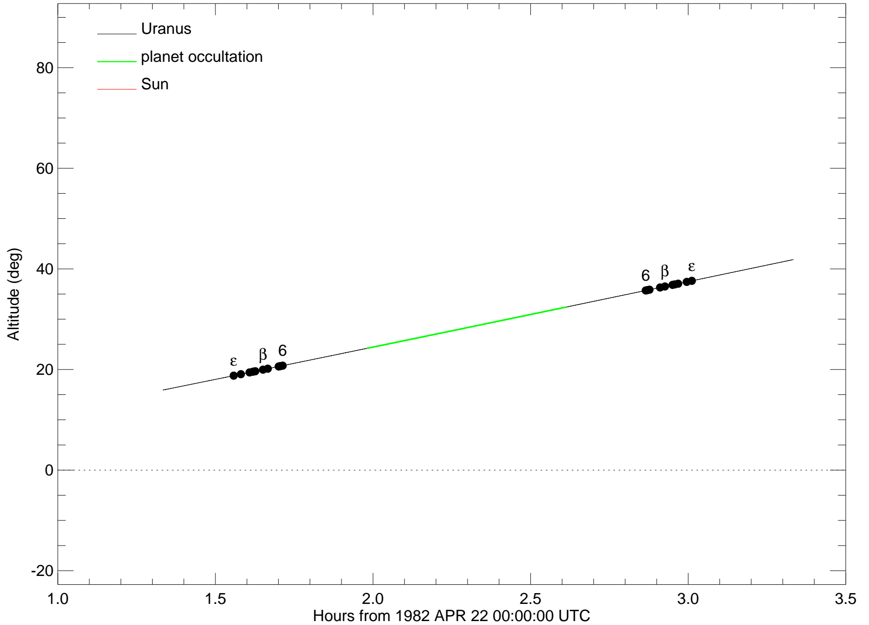
u14 observed from Las Campanas Observatory 250cm
