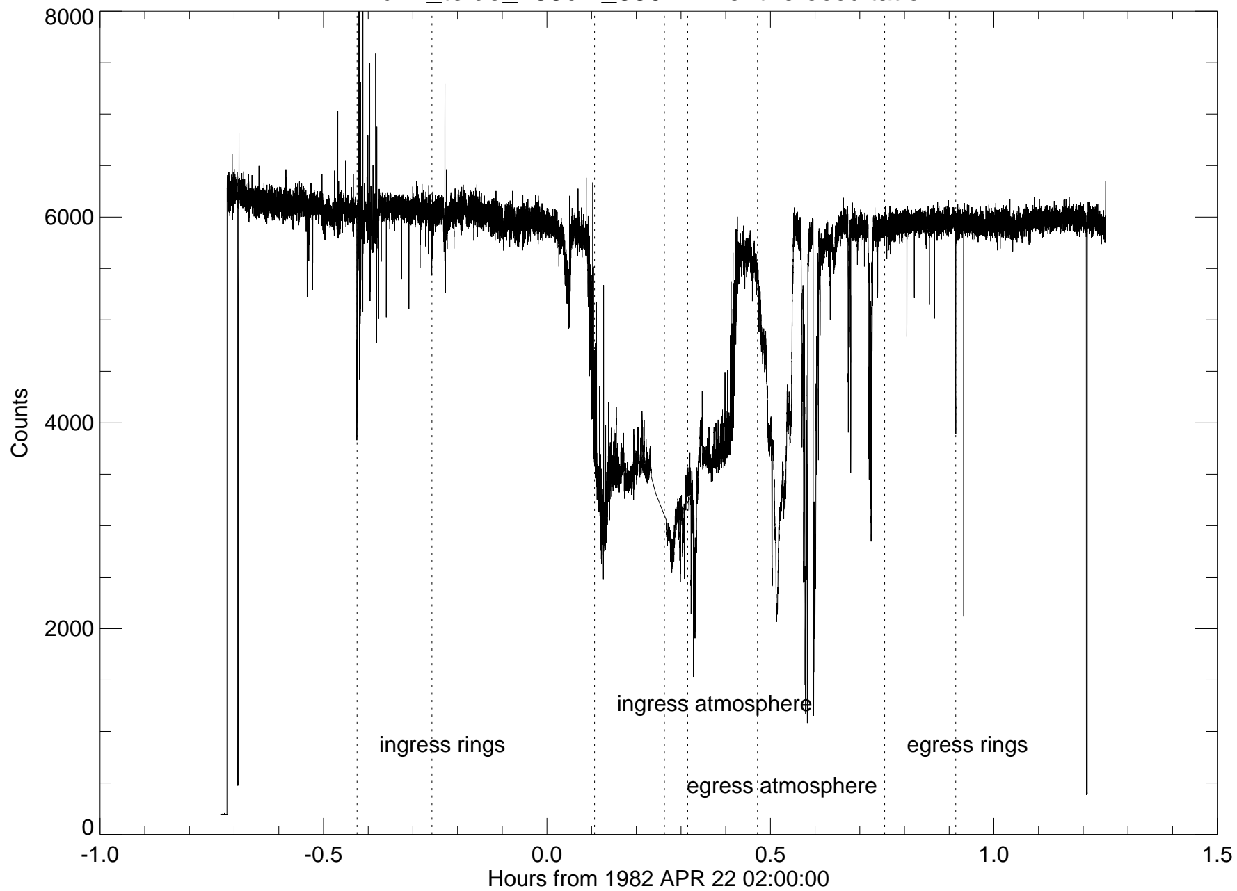
u14_teide_155cm_880nm - entire occultation
