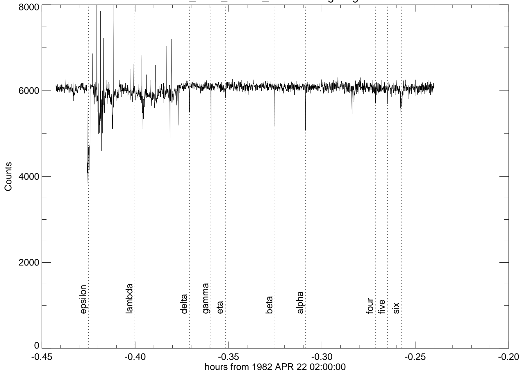
u14_teide_155cm_880nm - rings ingress
