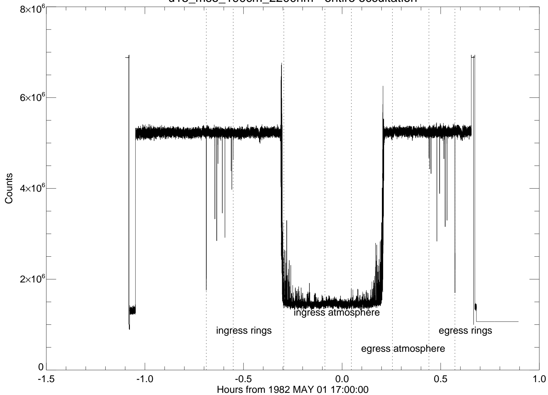
u15_mso_190cm_2200nm - entire occultation
