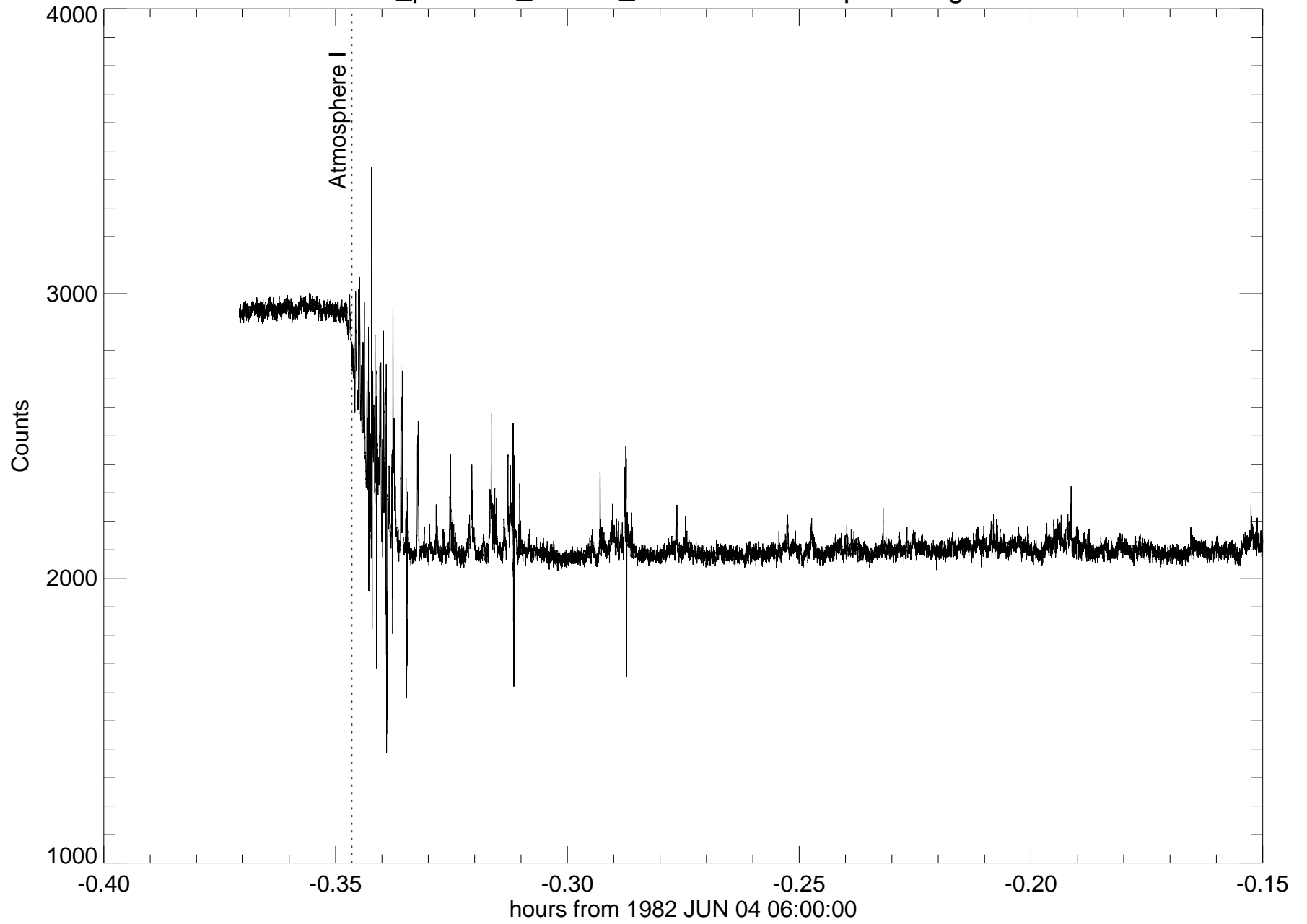
u16_palomar_508cm_2200nm - atmosphere ingress
