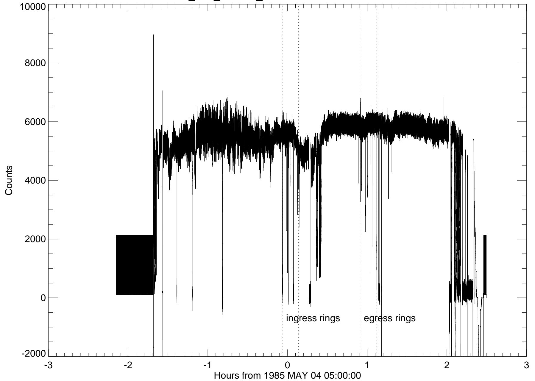
u23_ctio_400cm_2200nm - entire occultation
