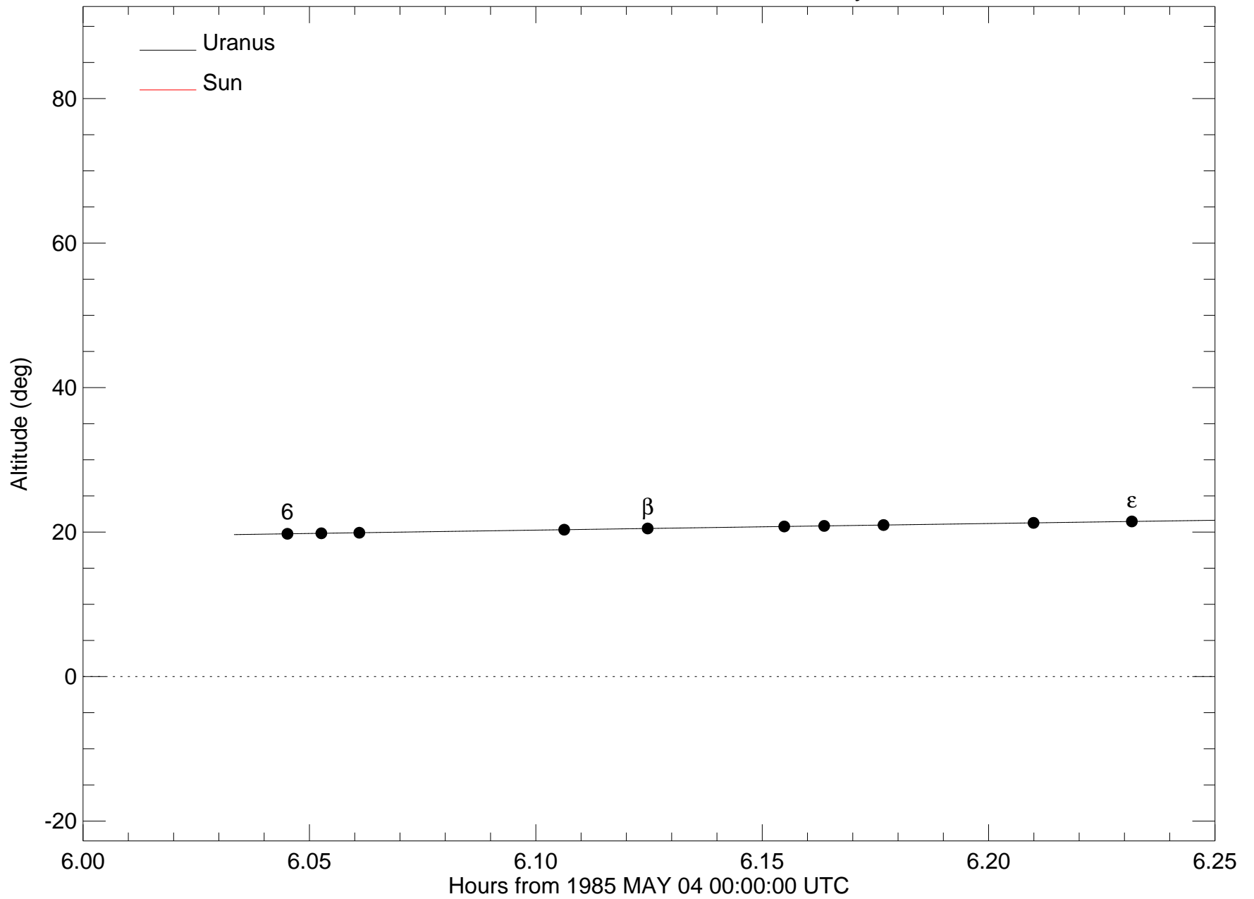
u23 observed from McDonald Observatory 270cm
