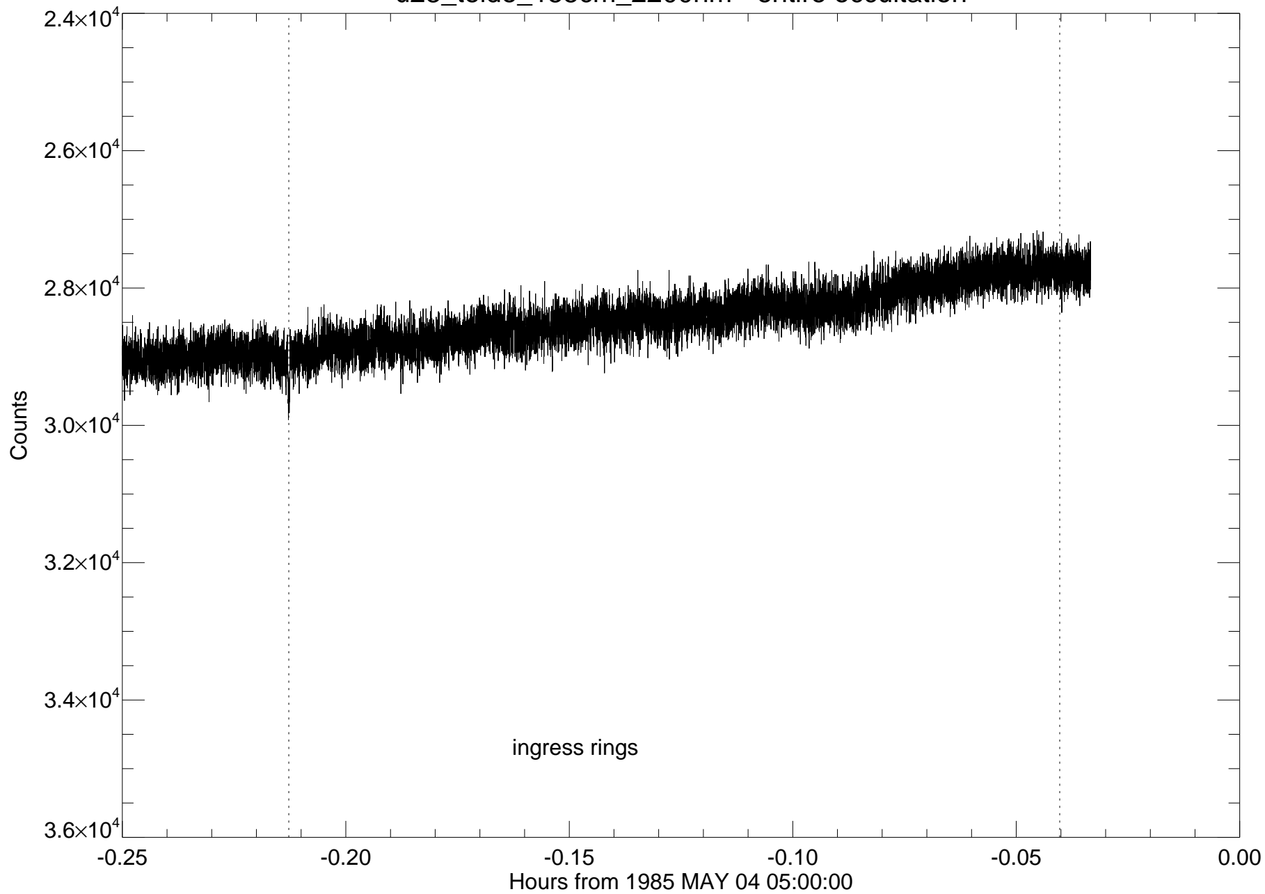
u23_teide_155cm_2200nm - entire occultation
