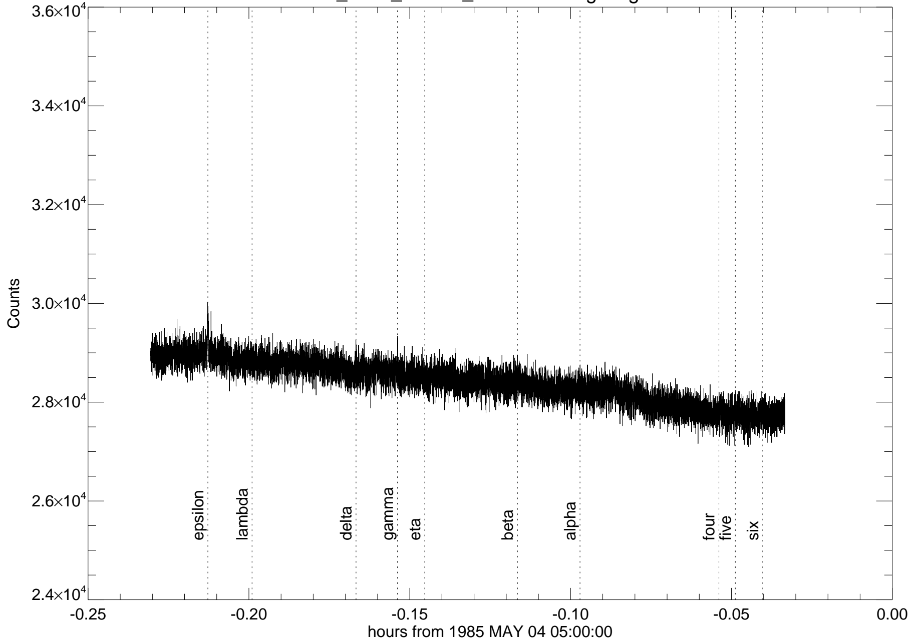
u23_teide_155cm_2200nm - rings ingress
