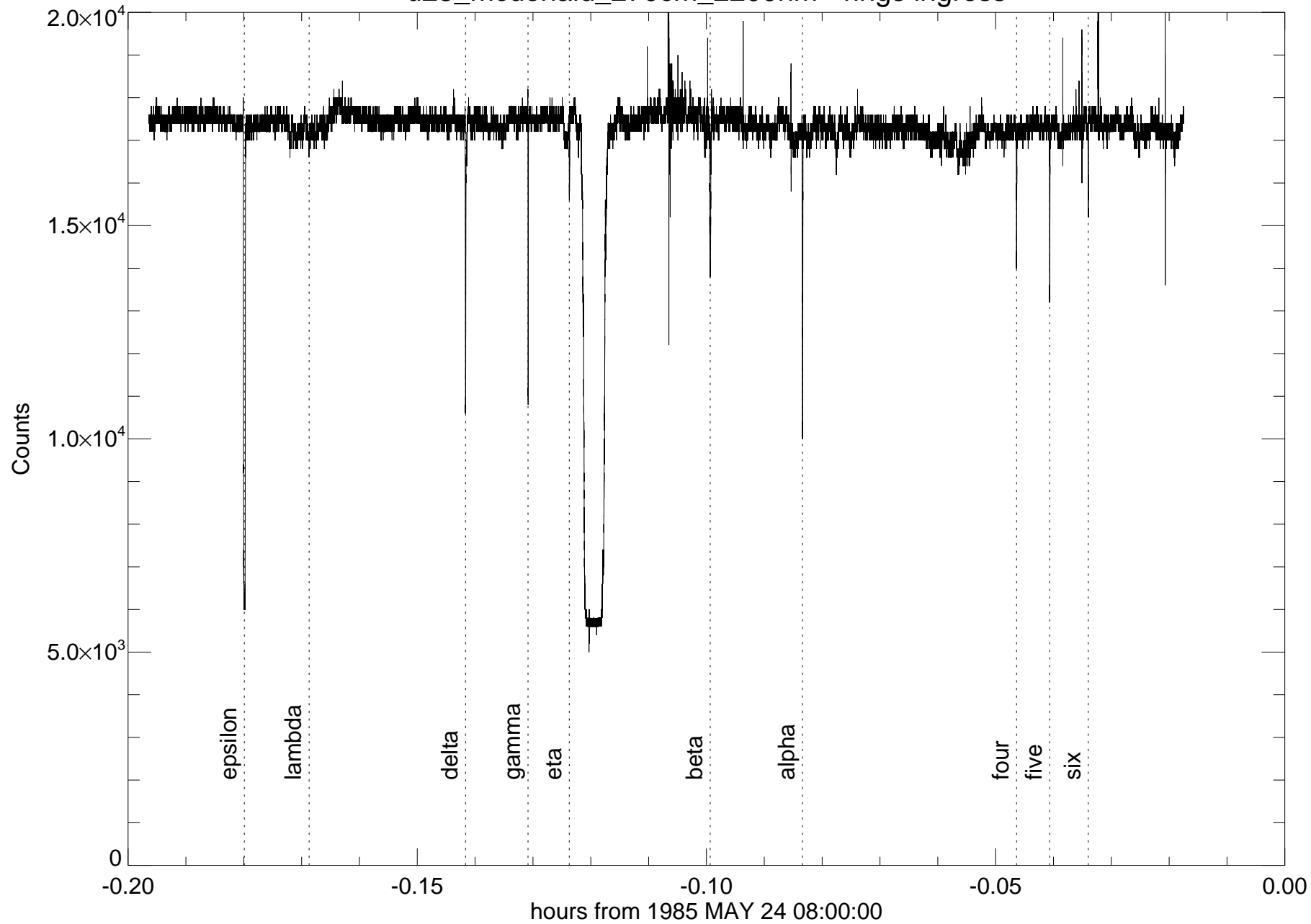
u25_mcdonald_270cm_2200nm - rings ingress
