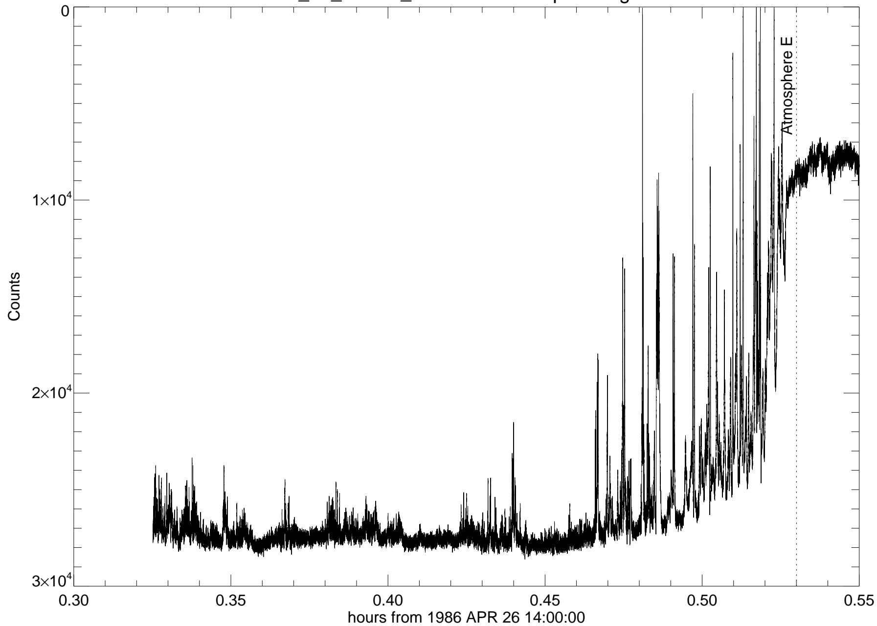
u28_irtf_320cm_2200nm - atmosphere egress
