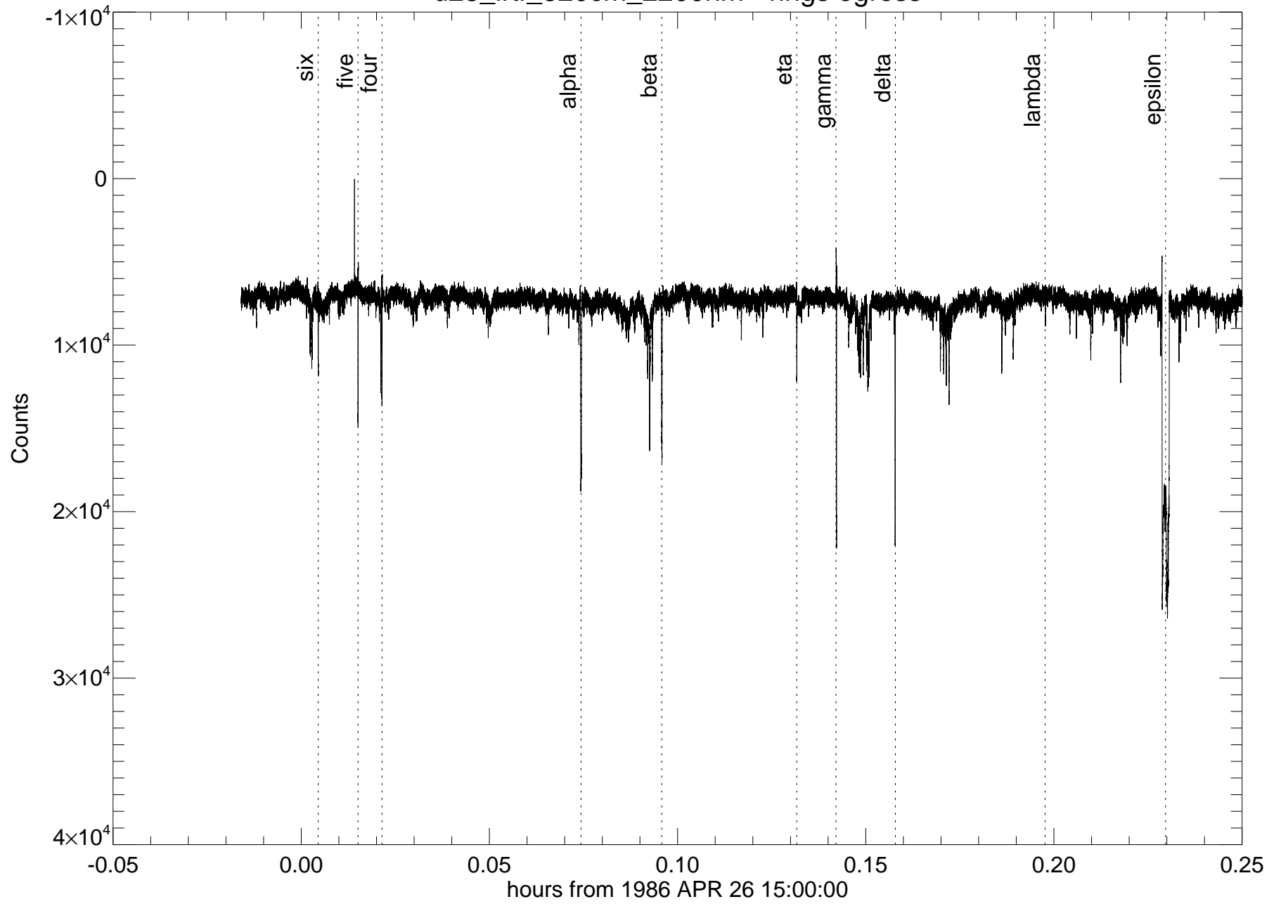
u28_irtf_320cm_2200nm - rings egress
