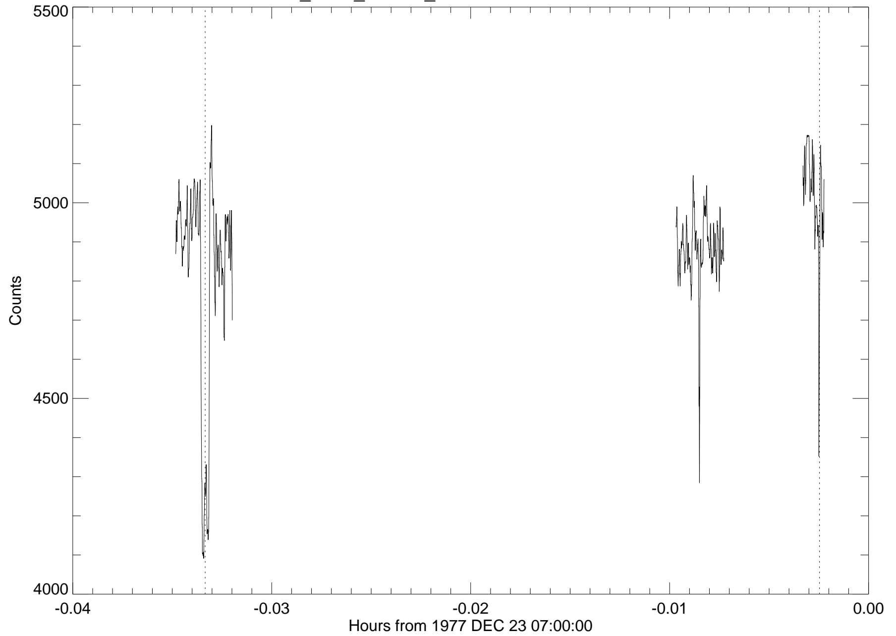
u2_teide_155cm_880nm - entire occultation
