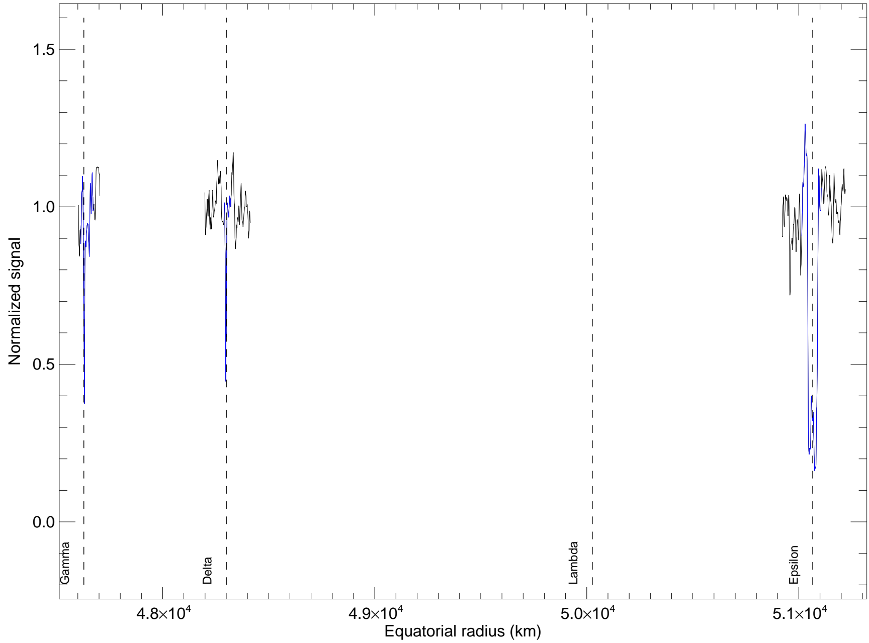
u2_teide_155cm_880nm rings ingress
