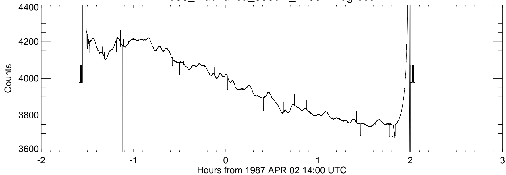
u36_maunakea_380cm_2200nm egress
