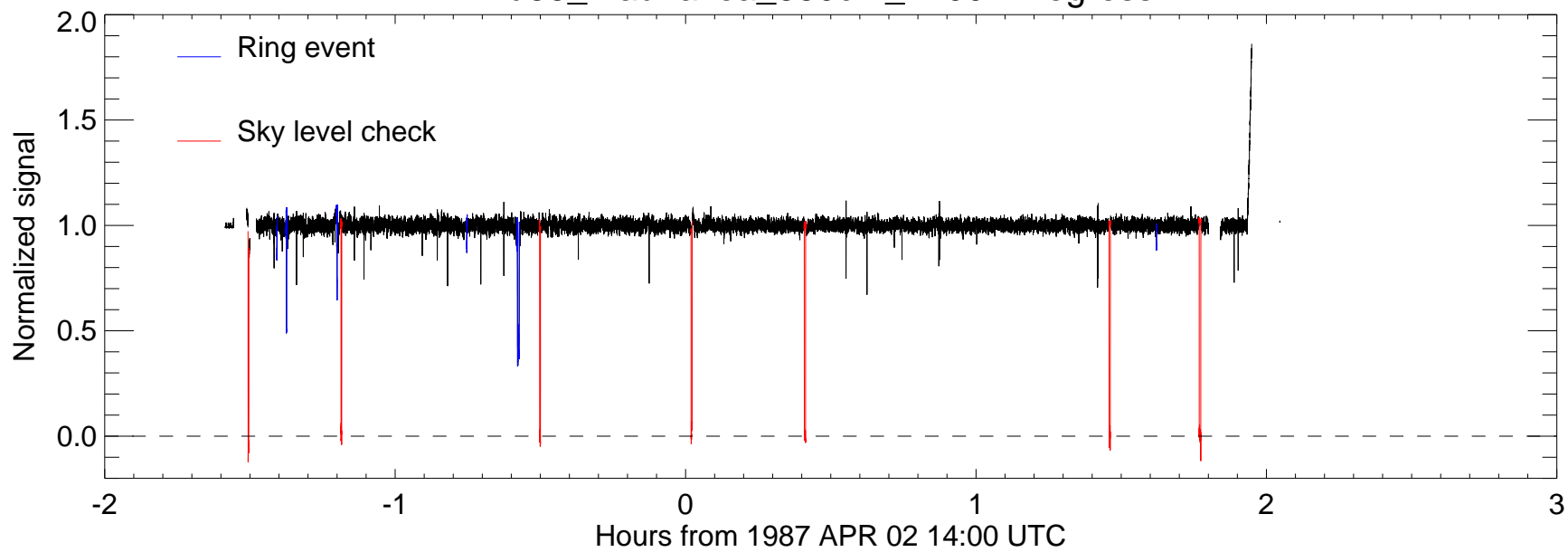
u36_maunakea_380cm_2200nm egress
