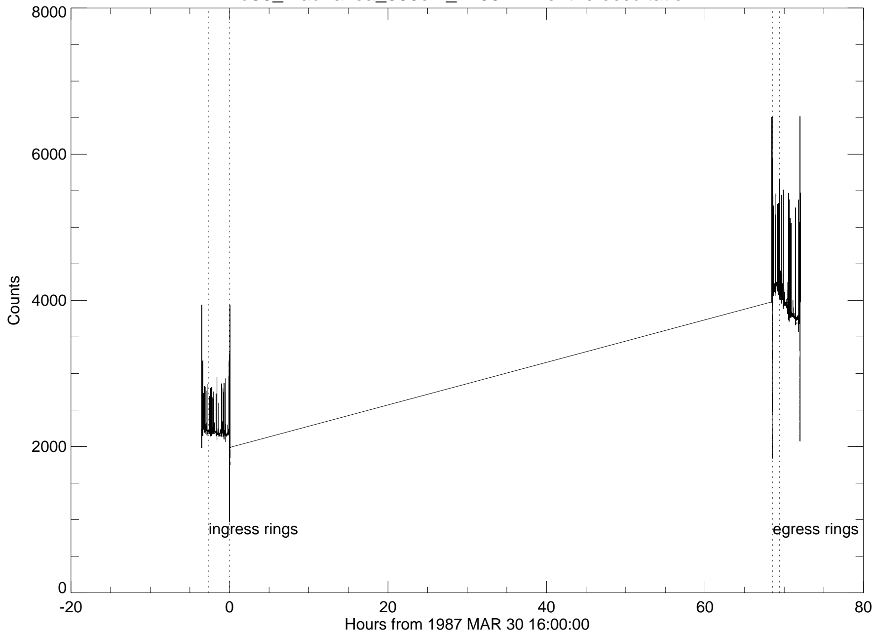
u36_maunakea_380cm_2200nm - entire occultation
