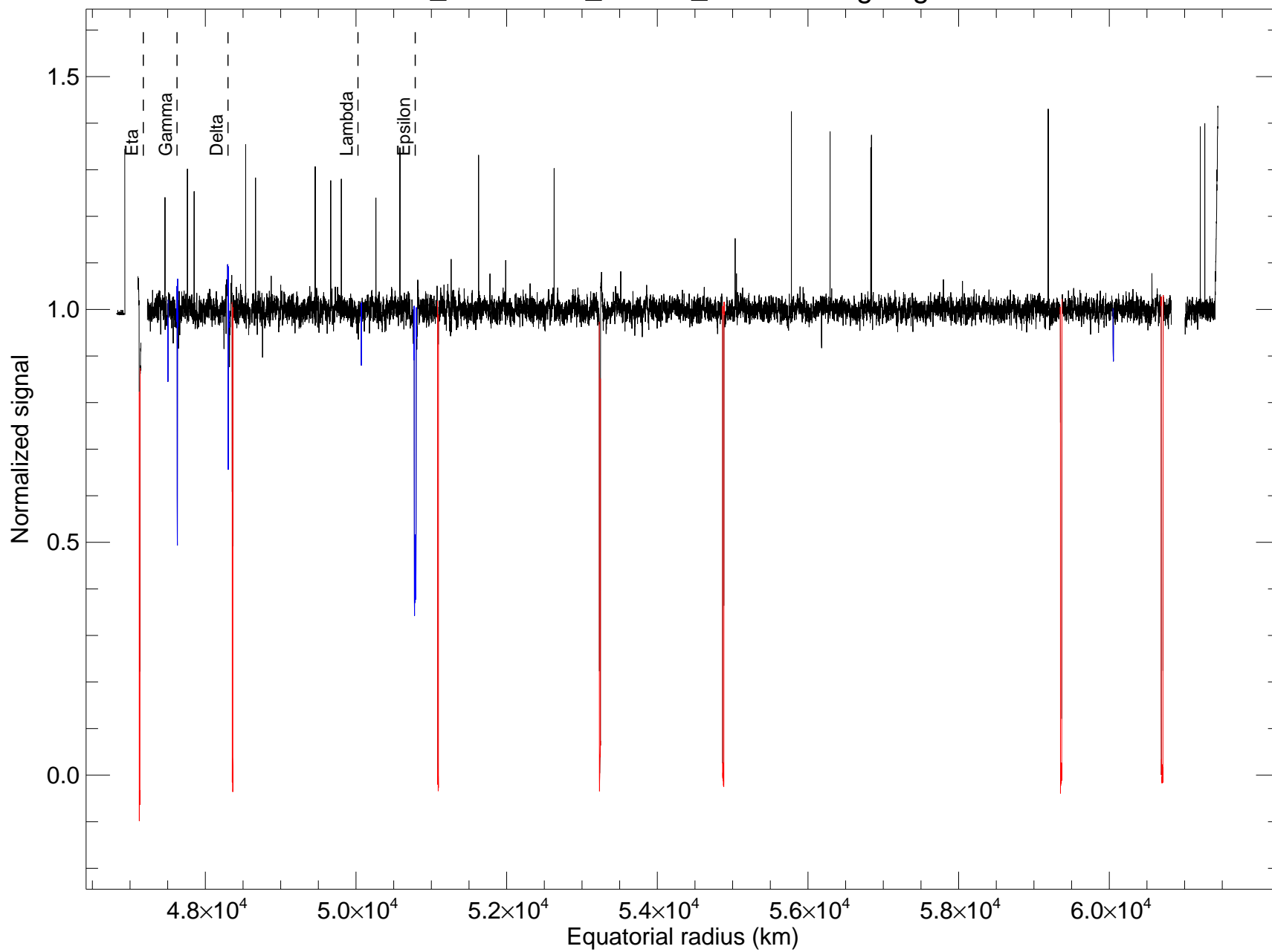
u36_maunakea_380cm_2200nm rings egress
