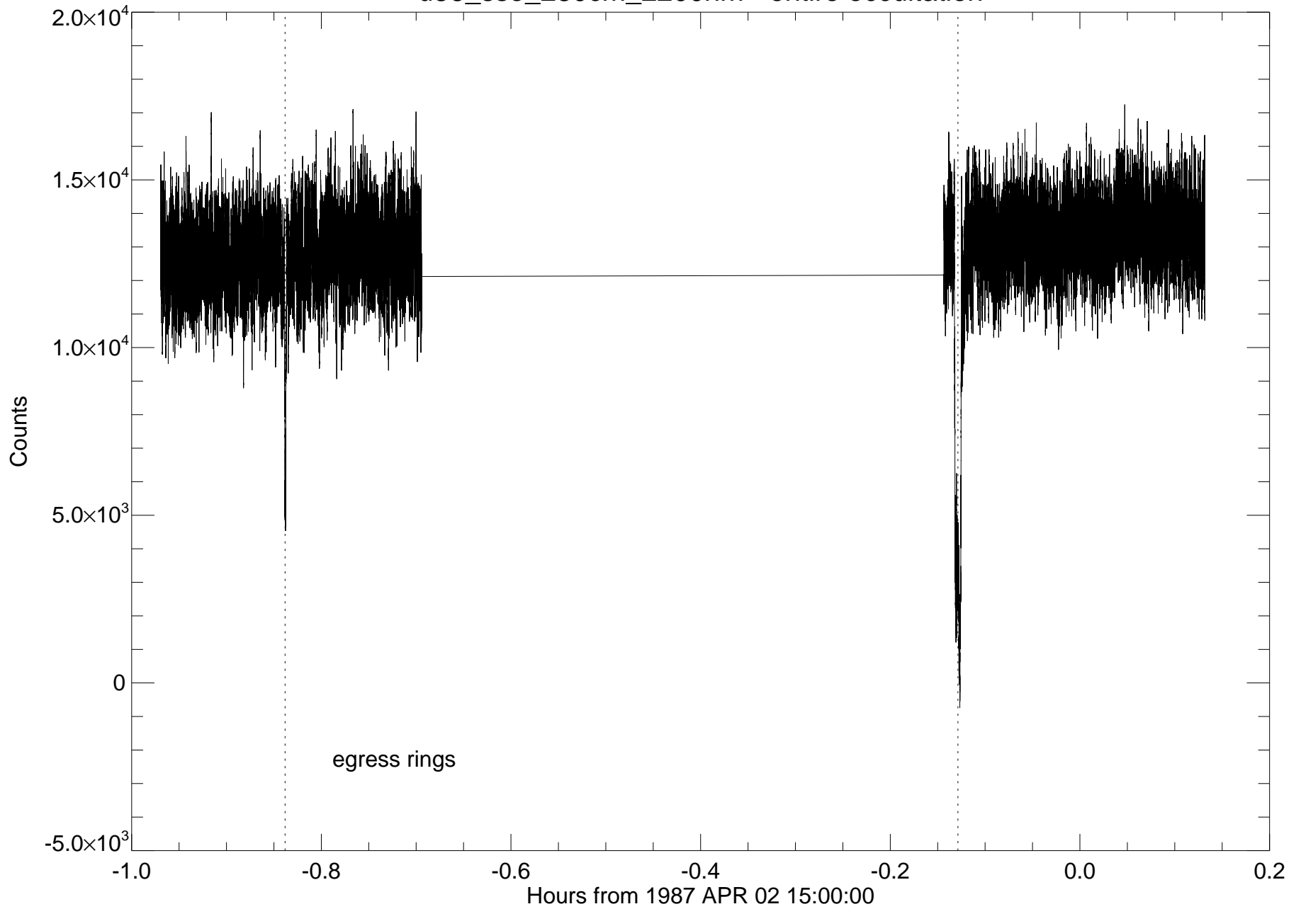
u36_sso_230cm_2200nm - entire occultation
