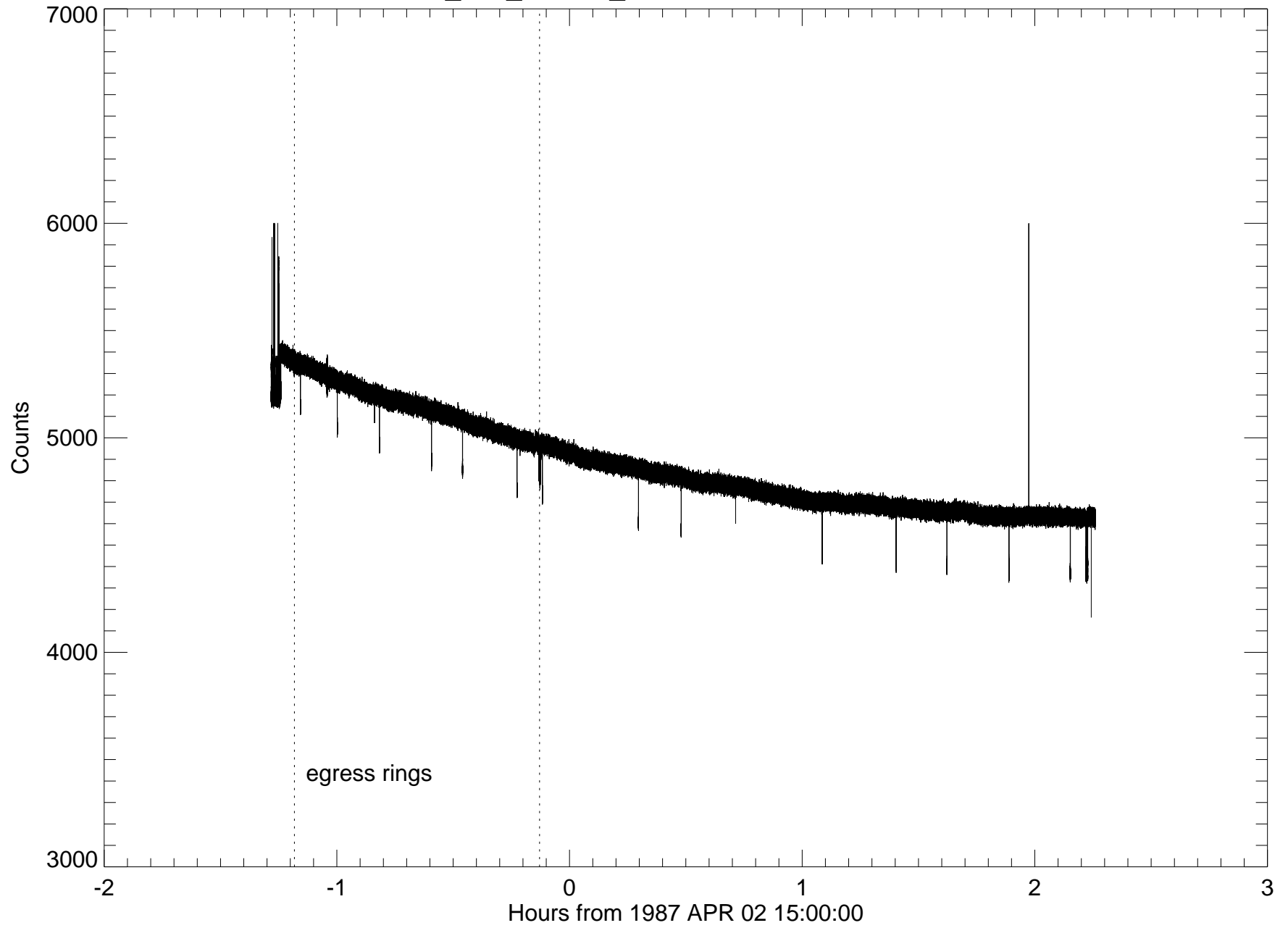
u36_sso_390cm_2200nm - entire occultation
