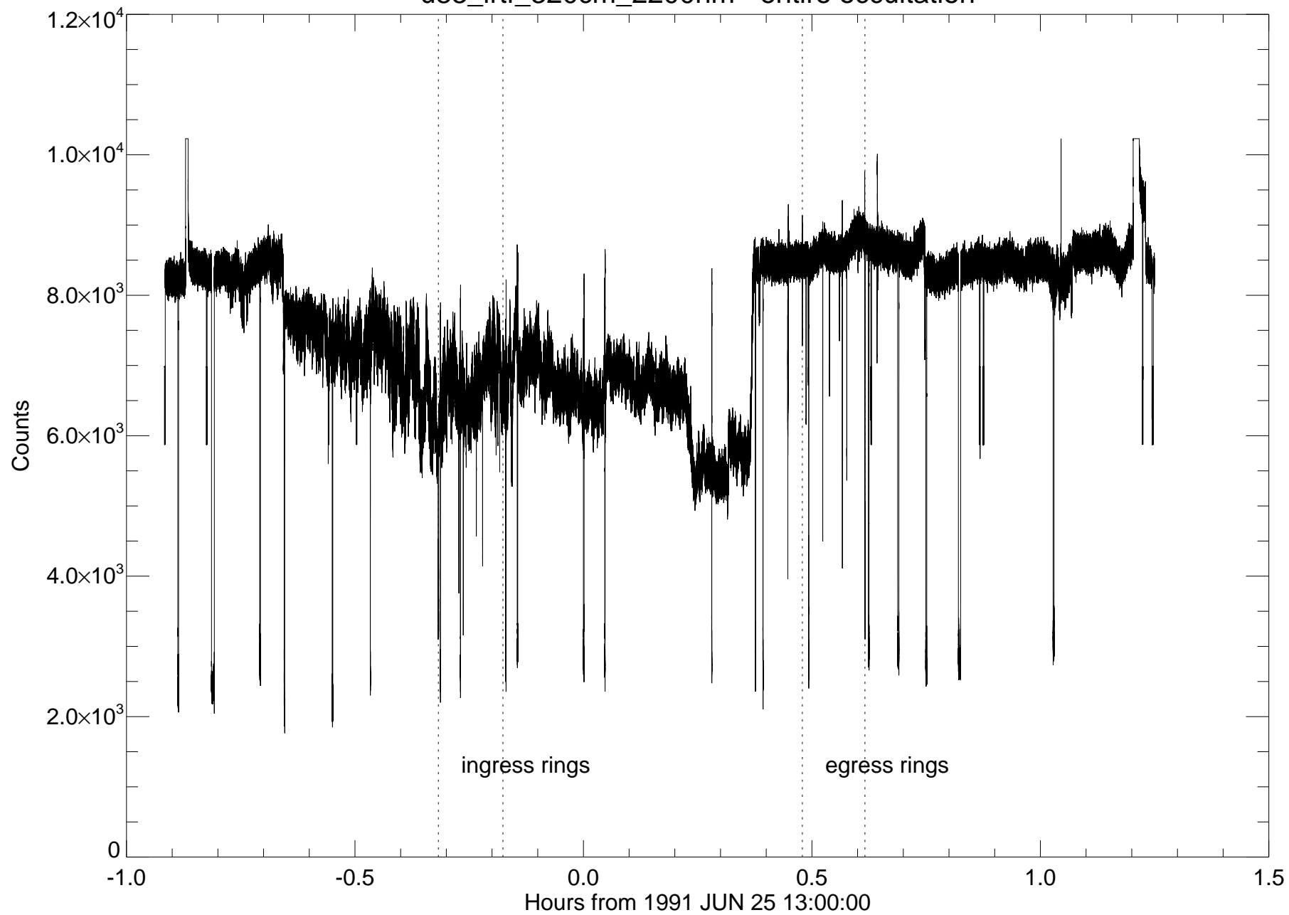
u83_irtf_320cm_2200nm - entire occultation
