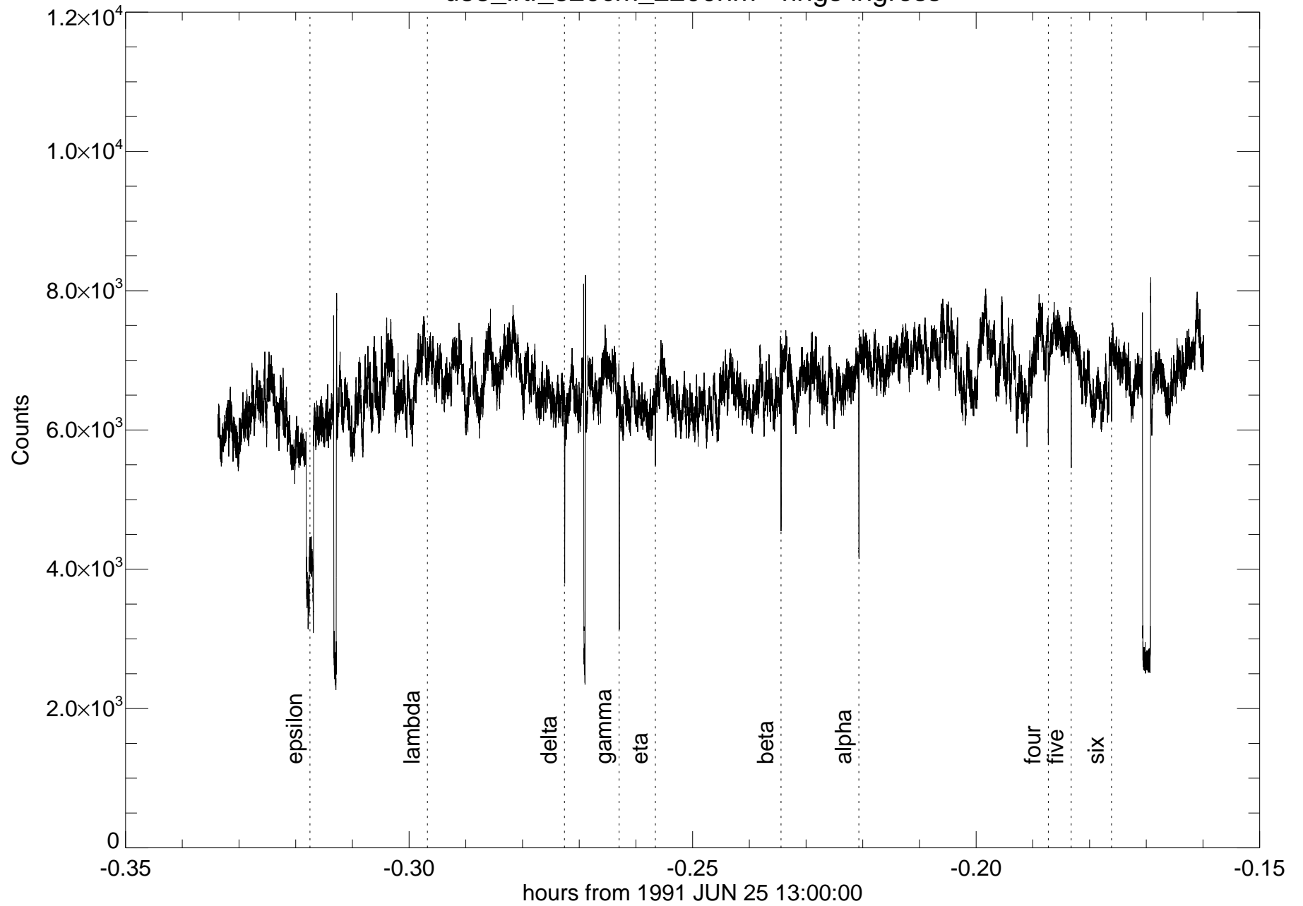
u83_irtf_320cm_2200nm - rings ingress
