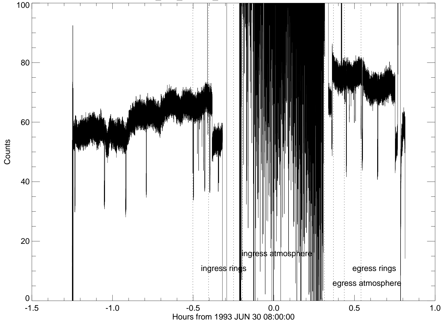
u9539_ctio_400cm_2200nm - entire occultation
