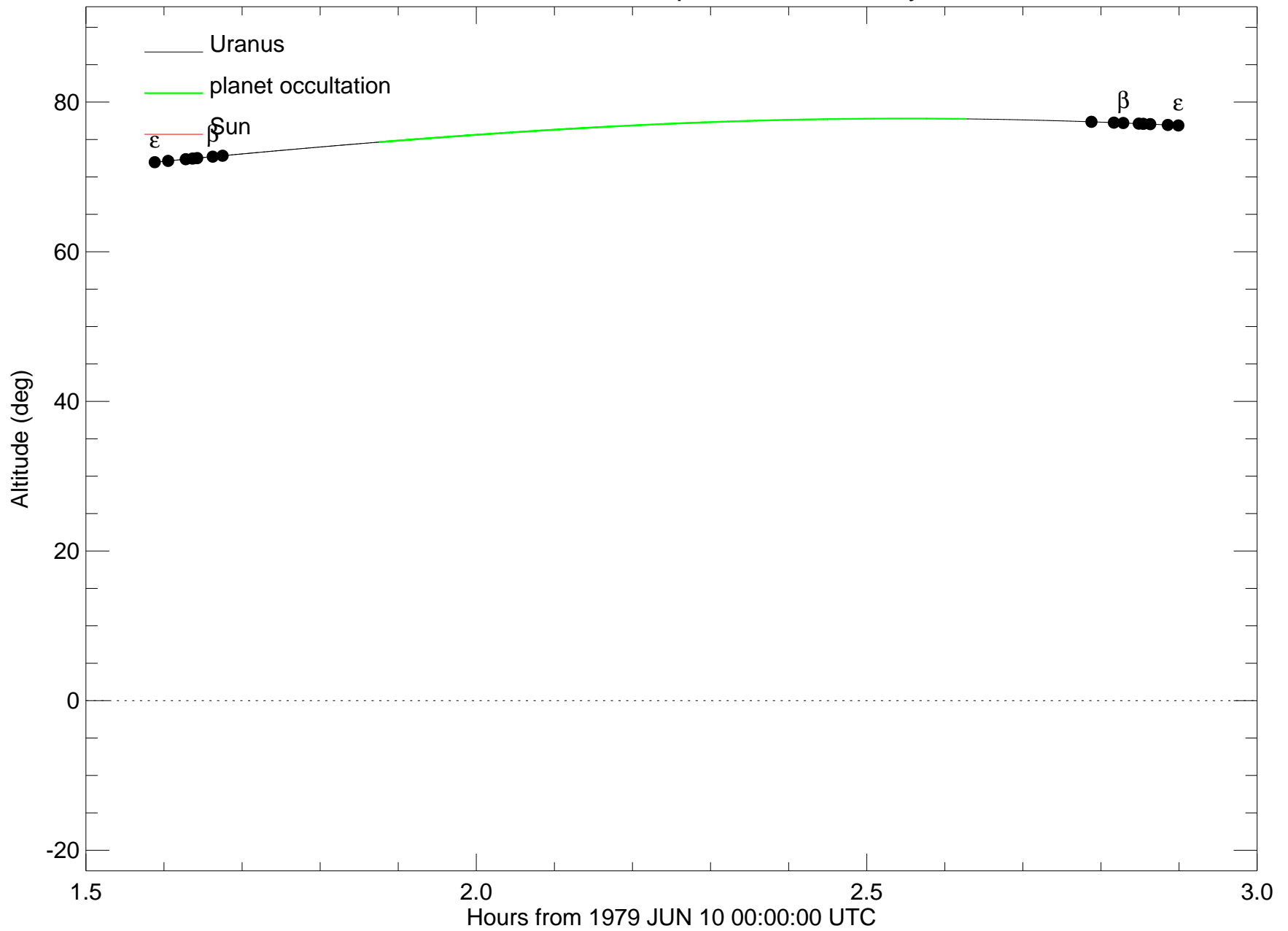
u9 observed from Las Campanas Observatory 250cm
