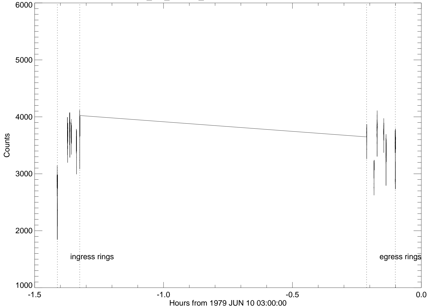
u9_lco_250cm_2200nm - entire occultation
