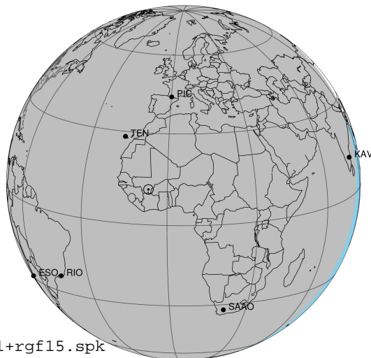
2023-10-24T00:09:30.3200 a: 02 38 15.1524 & +13 56 04.387 C/A ***** PA 342.24 deg v_sky -15.79 km/s D 03.99 AU Credit: Styled after SORA/Lucky Star
