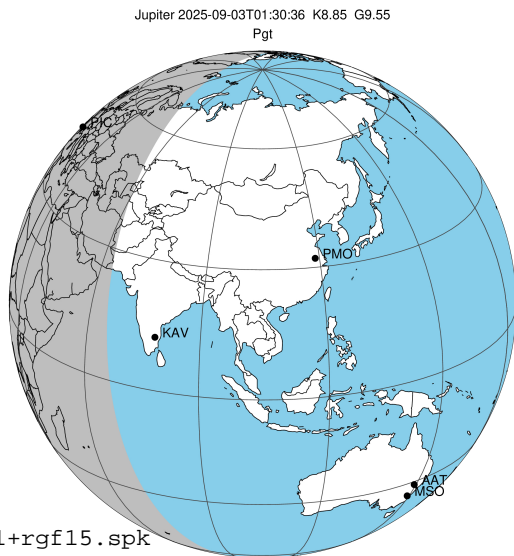
2025-09-03T01:30:36.2000 cc: 07 17 29.1942 s: +22 12 51.457 C/A 6.204" PA 187.04 deg v_sky +30.47 km/s D 05.72 AU Credit: Styled after SORA/Lucky Star
